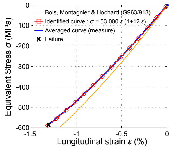
Figure 5: Non linear behavior in compression up to failure (woven carbon/epoxy material G939/M18)
