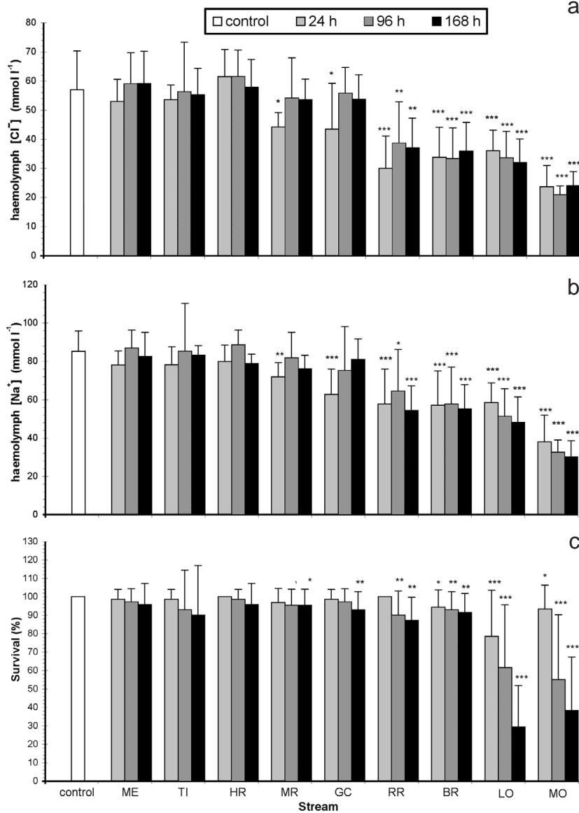
Fig. 2. Gammarus fossarum . Mean ( \pm SD) (a) haemolymph [\text{Cl}^-] , (b) haemolymph [\text{Na}^+] and (c) survival when exposed to granite bedrock stream. Significant differences against T_0 are indicated by asterisks (Student's t -test, * p < 0.05 ; ** p < 0.01 ; *** p < 0.001 )
