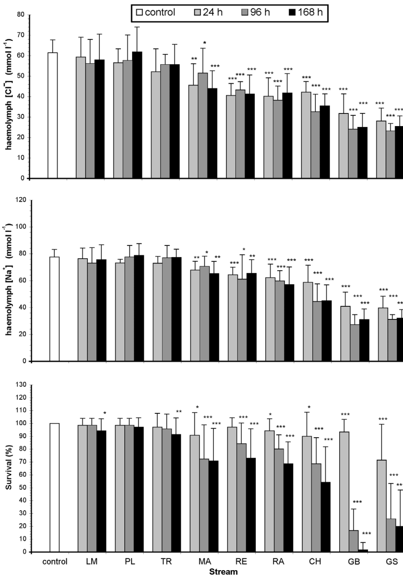
Fig. 3. Gammarus fossarum . Mean (±SD) (a) haemolymph [Cl - ], (b) haemolymph [Na + ] and (c) survival when exposed to sandstone bedrock stream. Significant differences against T 0 are indicated by asterisks (Student's t-test, *p < 0.05; **p < 0.01; ***p < 0.001)
