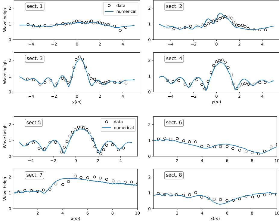
Figure 14: Periodic waves propagation over an elliptic shoal: Berkhoff experiments - Comparison of the computed mean wave height with the experimental data along the height wave gauges sections
