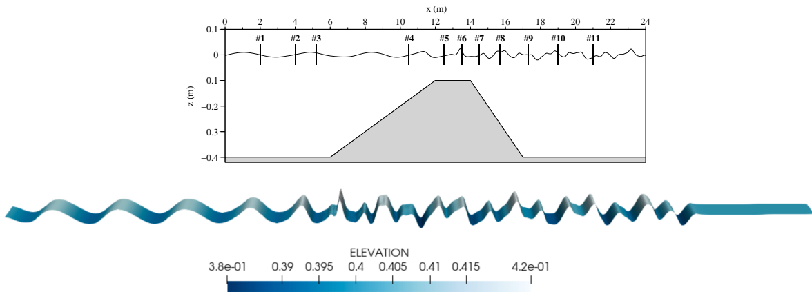
Figure 9: Propagation of periodic highly dispersive waves: the Dingemans experiments - Locations of wave gages and (rescaled) 3d view of the free surface during the propagation.
