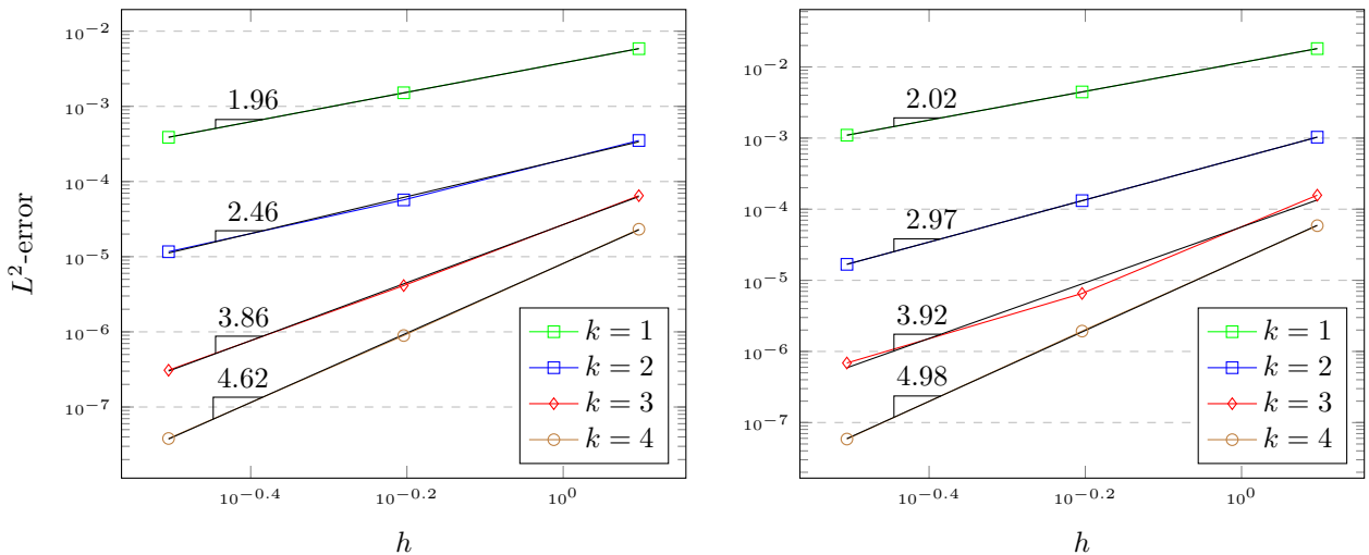
Figure 4: Solitary wave propagation over a flat bottom - L^2 -error for the free surface \eta (left) and the discharge q (right) vs. mesh size h for k = 1, 2, 3, 4 and r = k at t = 0.1 s.
