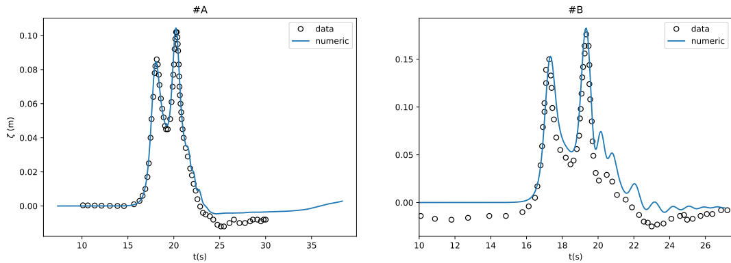
Figure 8: Shoaling and reflection of a solitary wave on a sloping beach: time series of the free surface at x = 17.75 \text{ m} for the \alpha -GN-LM model
