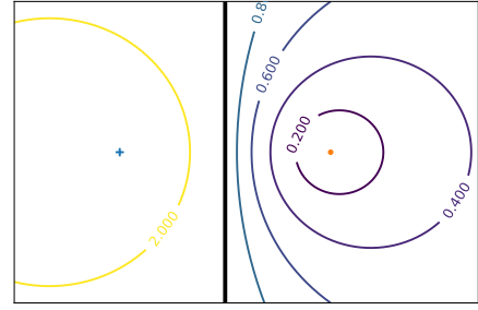
Fig. 2. Evolution of the decision boundary based on d_\gamma , for a 1-NN classifier, on a 2D dataset with one positive (resp. negative) instance represented by a blue cross (resp. orange point). The value of \gamma is given on each boundary ( \gamma = 1 on the thick line).
