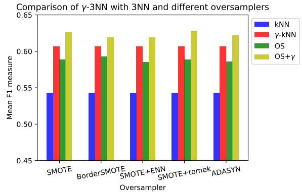
Fig. 4. Comparison of different sampling strategies averaged over the 19 public datasets. OS refers to the results of the corresponding sampling strategy and OS + \gamma to the case when the sampling strategy is combined with \gamma k -NN. k -NN and \gamma k -NN refers to the results of these methods without oversampling as obtained in Table II. (numerical values for these graphs are provided in supplementary material)
