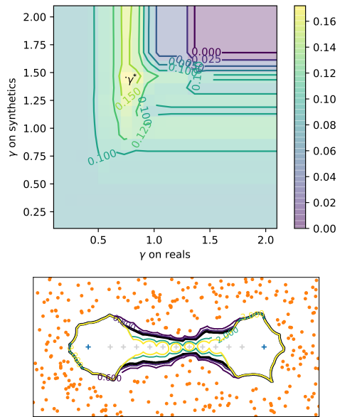
Fig. 5. (Top) An example of heatmap that shows the best couple of \gamma for the OS+ \gamma k -NN strategy on the yeast6 dataset with SMOTE and Tomek's link. (Bottom) Illustration, on a toy dataset, of the effect of varying the \gamma for generated positive points (in grey) while keeping a fixed \gamma = 0.4 for real positive points.
