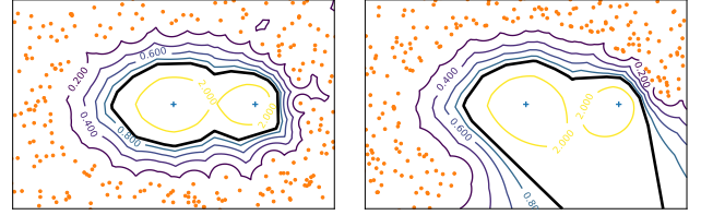
Fig. 3. Behavior of the decision boundary according to the \gamma value for the 1-NN classifier on two toy datasets. The positive points are represented by blue crosses and the negatives by orange points. The black line represents the standard decision boundary for the 1-NN classifier, i.e. when \gamma = 1 .
