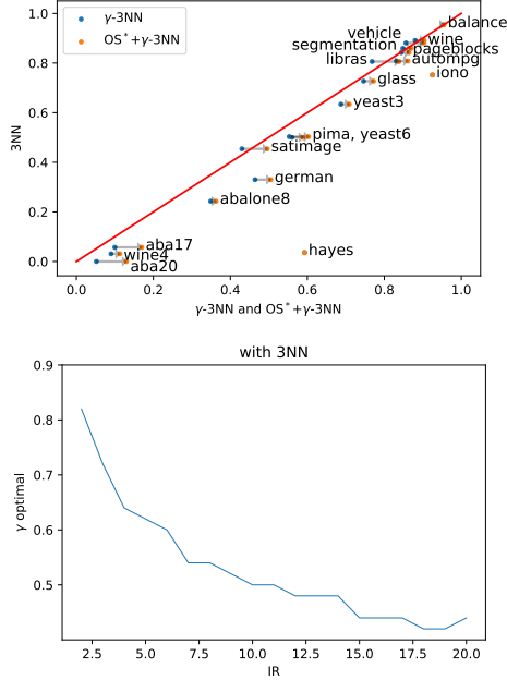
Fig. 6. (Top) Comparison of k -NN with (i) \gamma k -NN (points in blue) and (ii) \gamma k -NN coupled with the best sampling strategy (OS*) (points in orange) for each dataset and for k = 3 . Points below the line y = x means that k -NN is outperformed. (Bottom) Evolution of the optimal \gamma value with respect to the IR for k = 3 .
