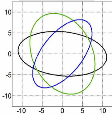
[A] supFig 1
