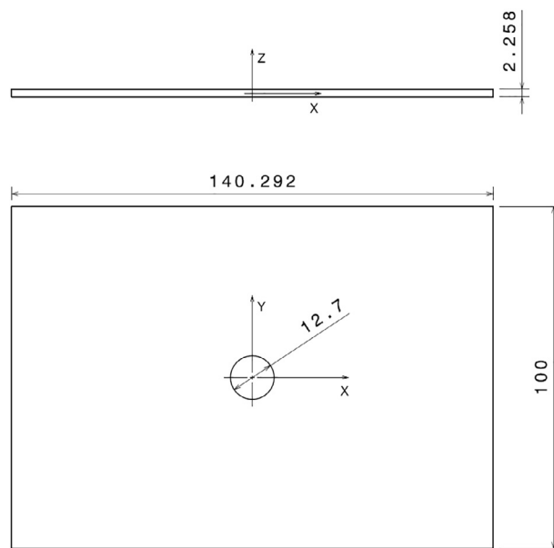
Fig. 1. Geometry of the multilayer composite plate (sizes in [mm]).
