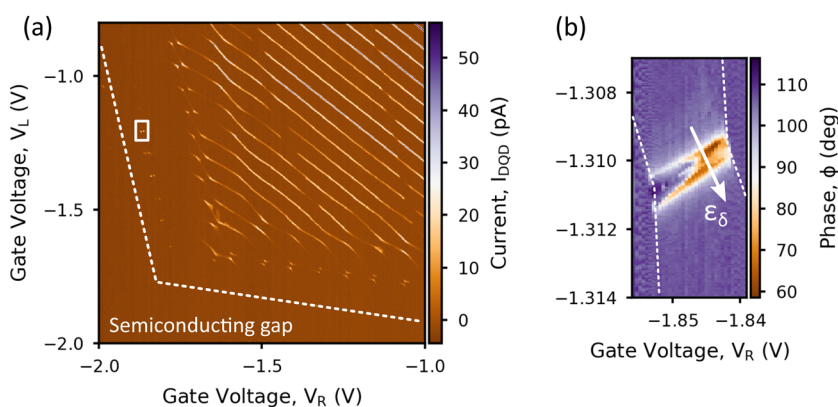
Fig. 2 Carbon nanotube double quantum dot in the few electron regime. a Stability diagram of our double quantum dot spin qubit, given by the current I through the double dot versus the gate voltages V_L and V_R . The gap is at the lower left corner of the stability diagram and is indicated by white dashed lines. b Phase contrast for the transmitted microwave signal along a charge degeneracy line in the region indicated by the white square in (a)
