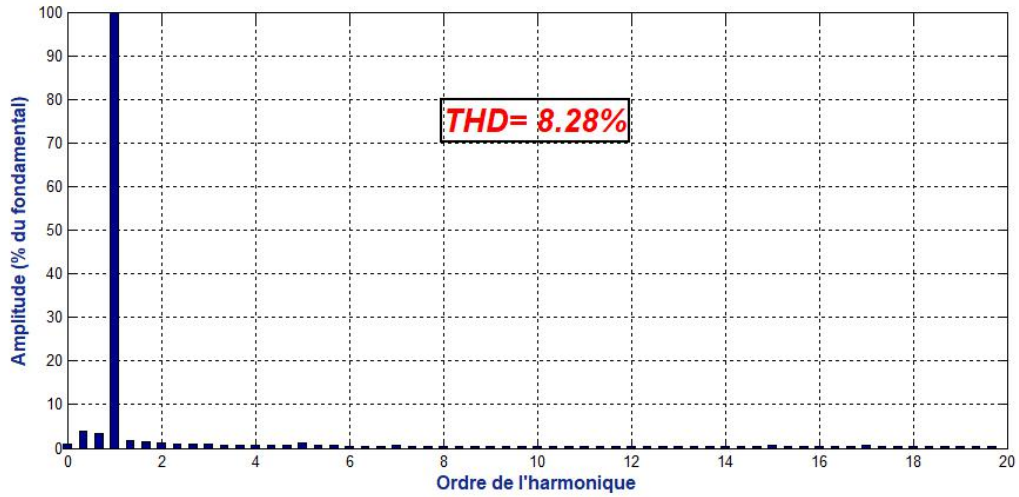
Fig. 12. Spectrum of the current after filtering for t = 0 s.
