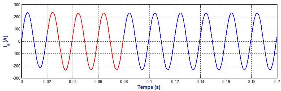
Fig. 13. Network current after filtering ( t = 0.02 s)
