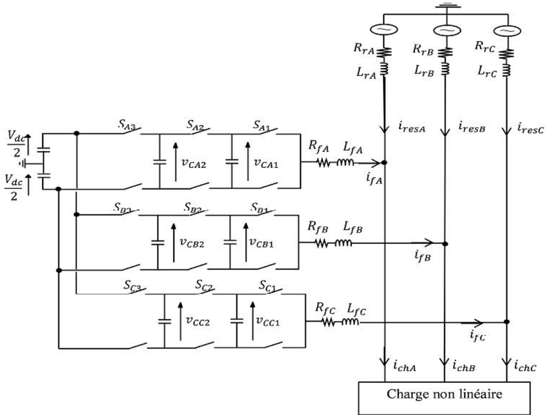
Fig. 3. Active filter based on a three phase multicell inverter
