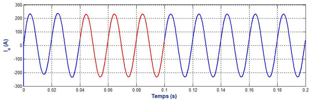
Fig. 15. Network current after filtering ( t = 0.04\text{s} )
