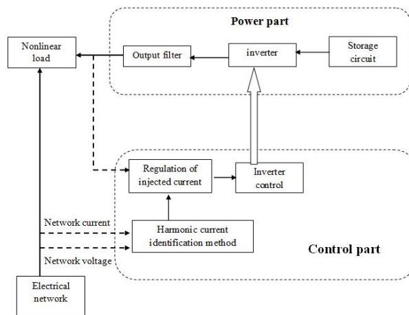
Fig. 2. General structure of an active filter
