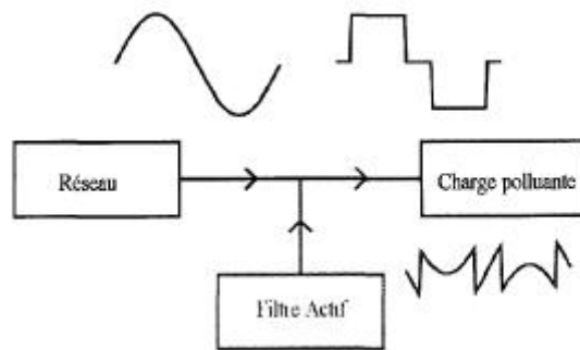
Fig. 1. Active filter principle
