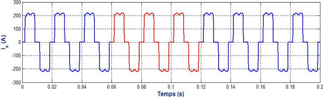
Fig. 7. Current waveform before filtering.
