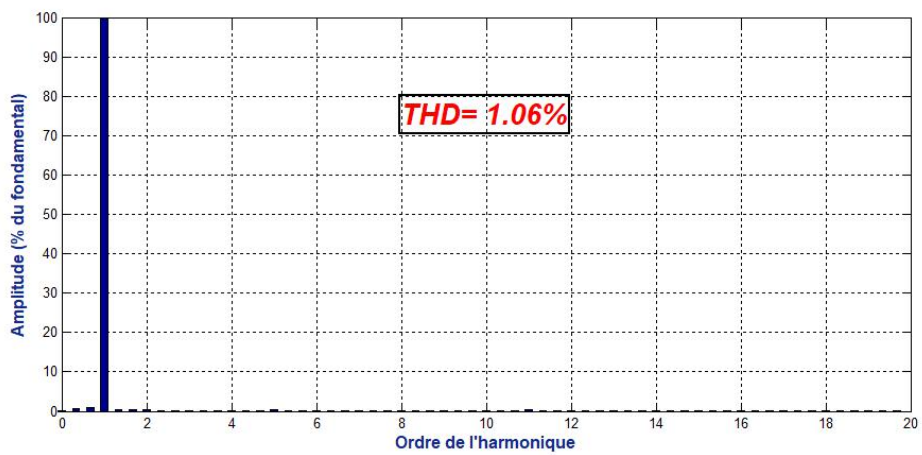
Fig. 14. Spectrum of the current after filtering for t = 0.02 s
