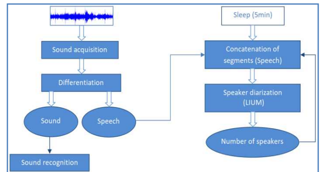
Figure 1. Application architecture.
