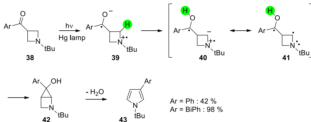
Scheme 8. Synthesis of pyrroles from azetidiny ketones via 1,4-hydrogen abstraction.
