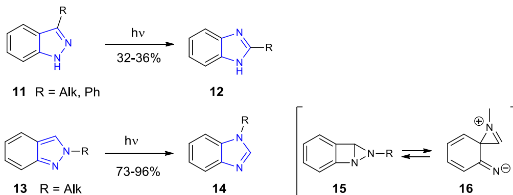
Scheme 2. Photochemical rearrangement of benzopyrazol derivatives into corresponding benzoimidazol derivatives. The irradiation has been carried out with high pressure Hg-vapor lamps.
