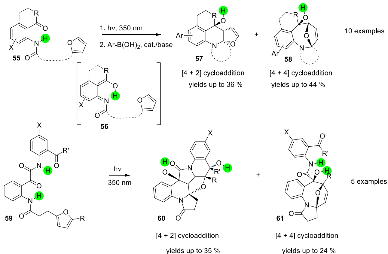
Scheme 12. Formation of polyheterocycles via photoenolisation.
