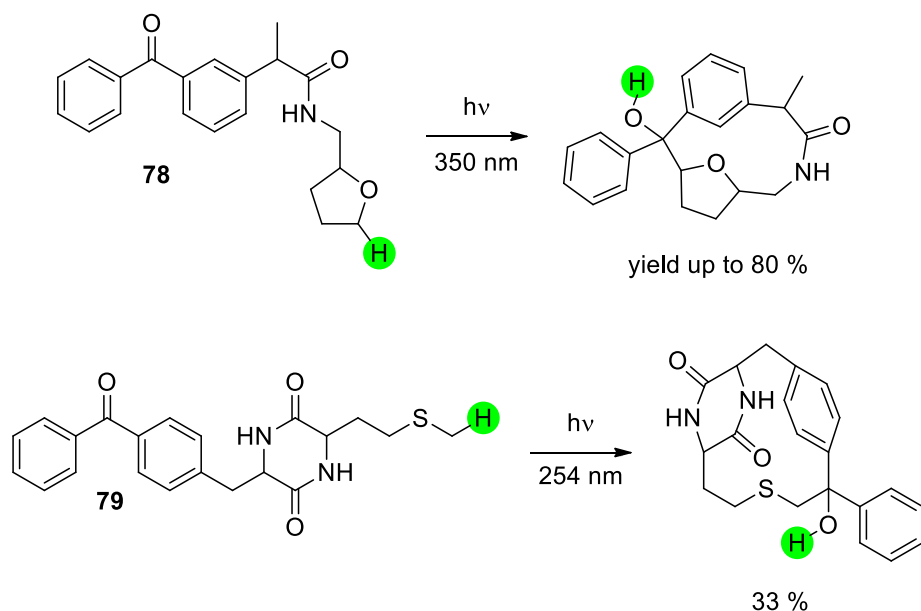
Scheme 18. Examples of 1,12-HAT and 1,15-HAT for macrocyclization.
