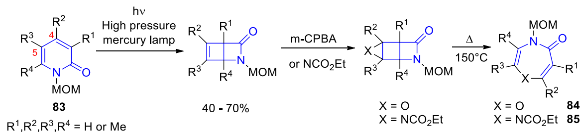
Scheme 21. Synthesis of 7 membered heterocycles using the photochemical electrocyclicization of pyridines.
