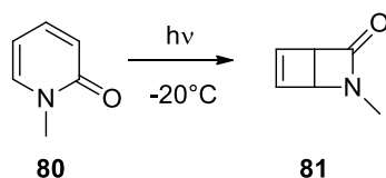
Scheme 19. Photochemical electrocyclization N-methylpyridone 80 .
