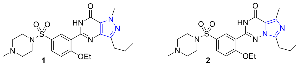
Figure 1. The pyrazol derivative 1 possesses a higher activity than the corresponding imidazole derivative 2 .
