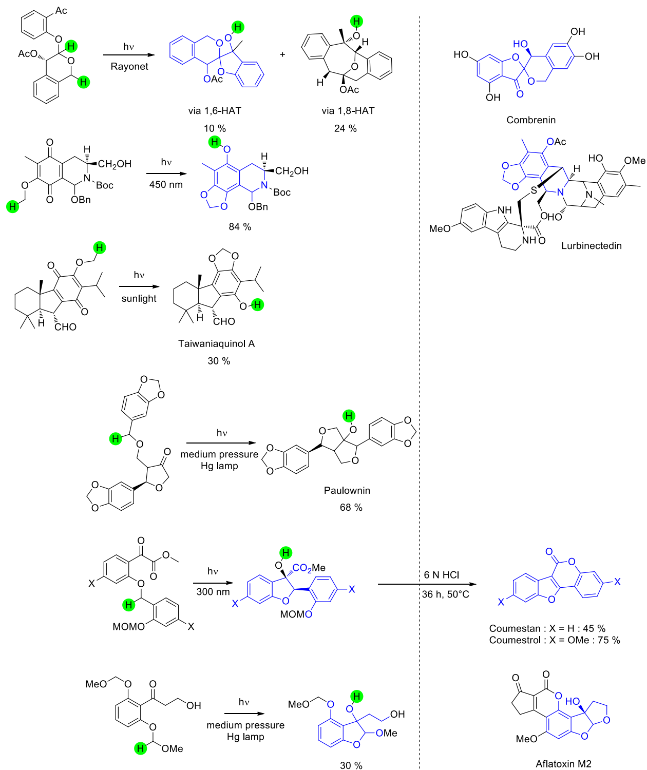
Scheme 16. Synthesis of various precursors of natural products via 1,6-HAT.
