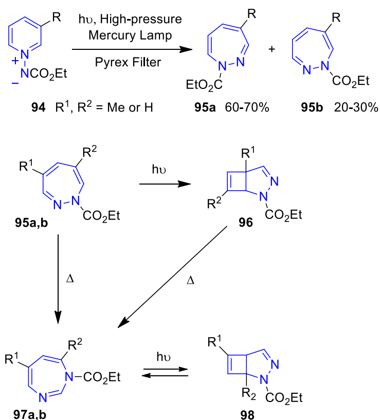
Scheme 24. Photochemical and thermal reactions starting with pyridine N-imides.
