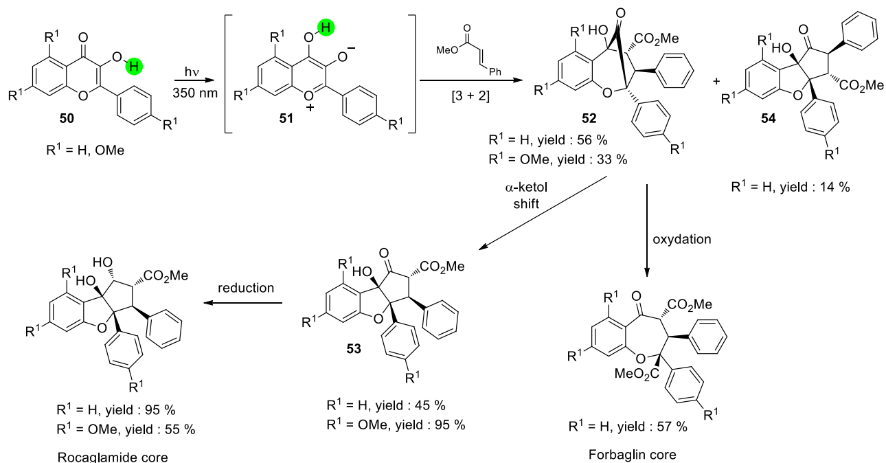
Scheme 10. Formation of bioactive natural compounds core of forbaglin and rocaglamide via 1,4-HAT and [3 + 2] cycloaddition.
