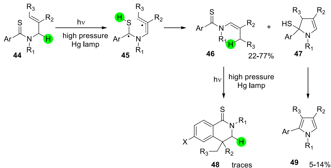
Scheme 9. Synthesis of pyrroles from thioamides derivatives.
