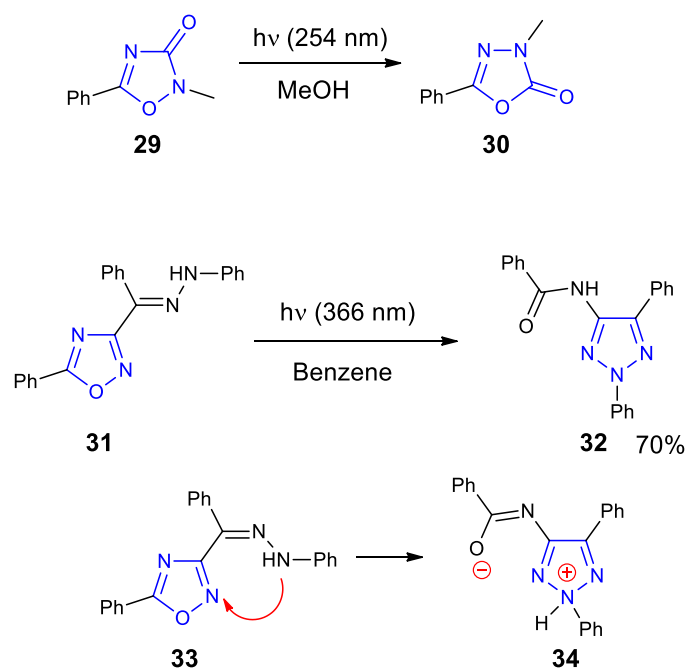
Scheme 6. Photochemical rearrangements with isoxadiazole derivatives.
