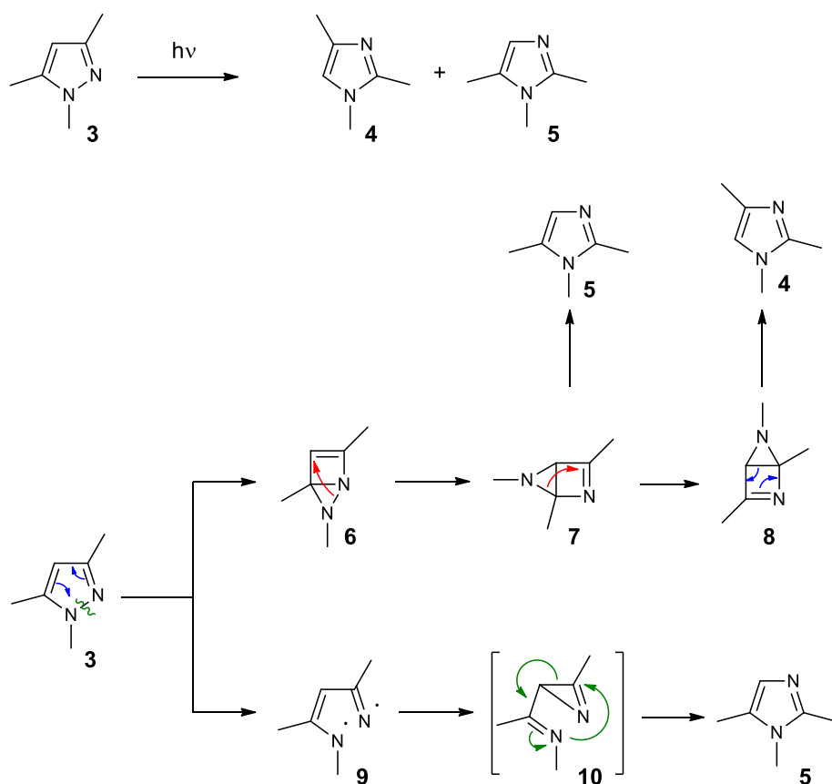
Scheme 1. Photochemical transformation of a pyrazol derivative into imidazoles.
