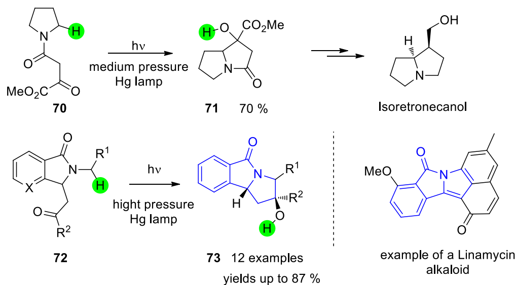
Scheme 15. Access to Isoretronecanol and Linamycin core via 1,6-HAT.
