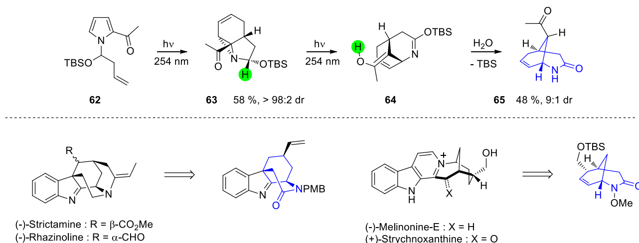
Scheme 13. Formation of a bridged azocanone: potential precursor for the synthesis of alkaloid structures.
