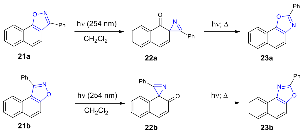
Scheme 4. Mechanistic study of the rearrangement of naphthisoaxazoles.
