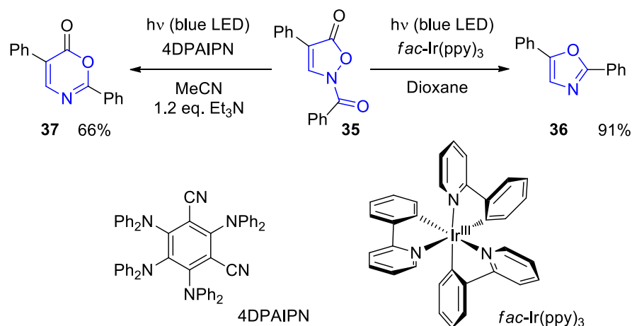
Scheme 7. Photoredox catalytic rearrangements of an isoxazolone derivative.
