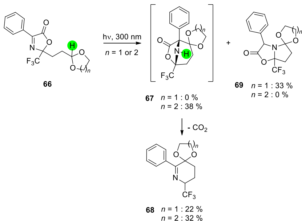
Scheme 14. Photoinduced intramolecular radical cyclisation via 1,5-HAT with imines.
