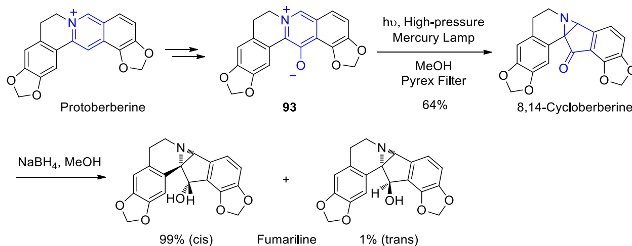
Scheme 23. Photochemical electrocyclicization applied to the synthesis of fumariline.
