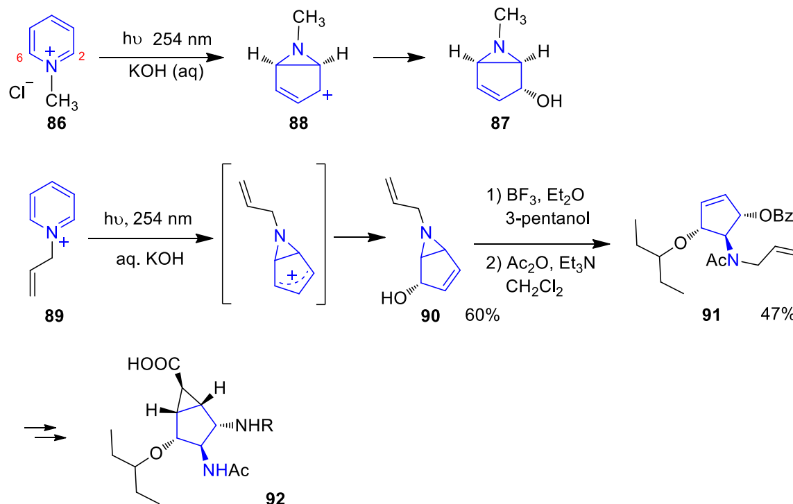
Scheme 22. Photochemical electrocyclicization of a pyridinium salts.
