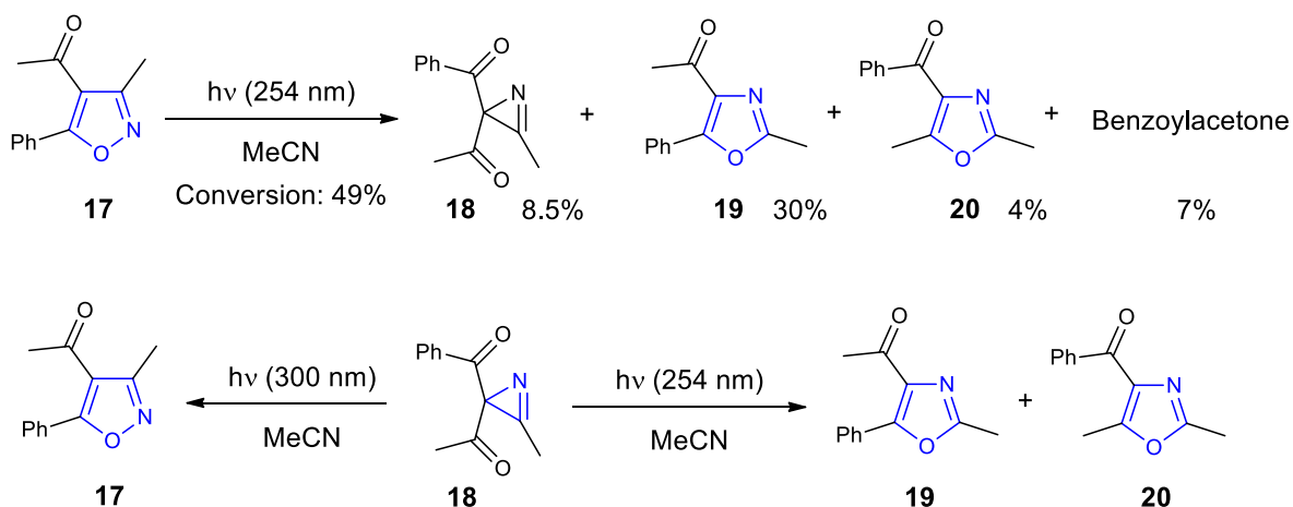
Scheme 3. Photochemical rearrangement of an isoxazol compound.
