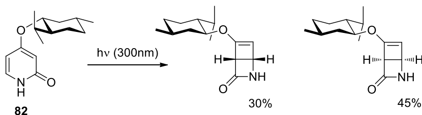
Scheme 20. Asymmetric electrocyclization of a pyridine derivative.
