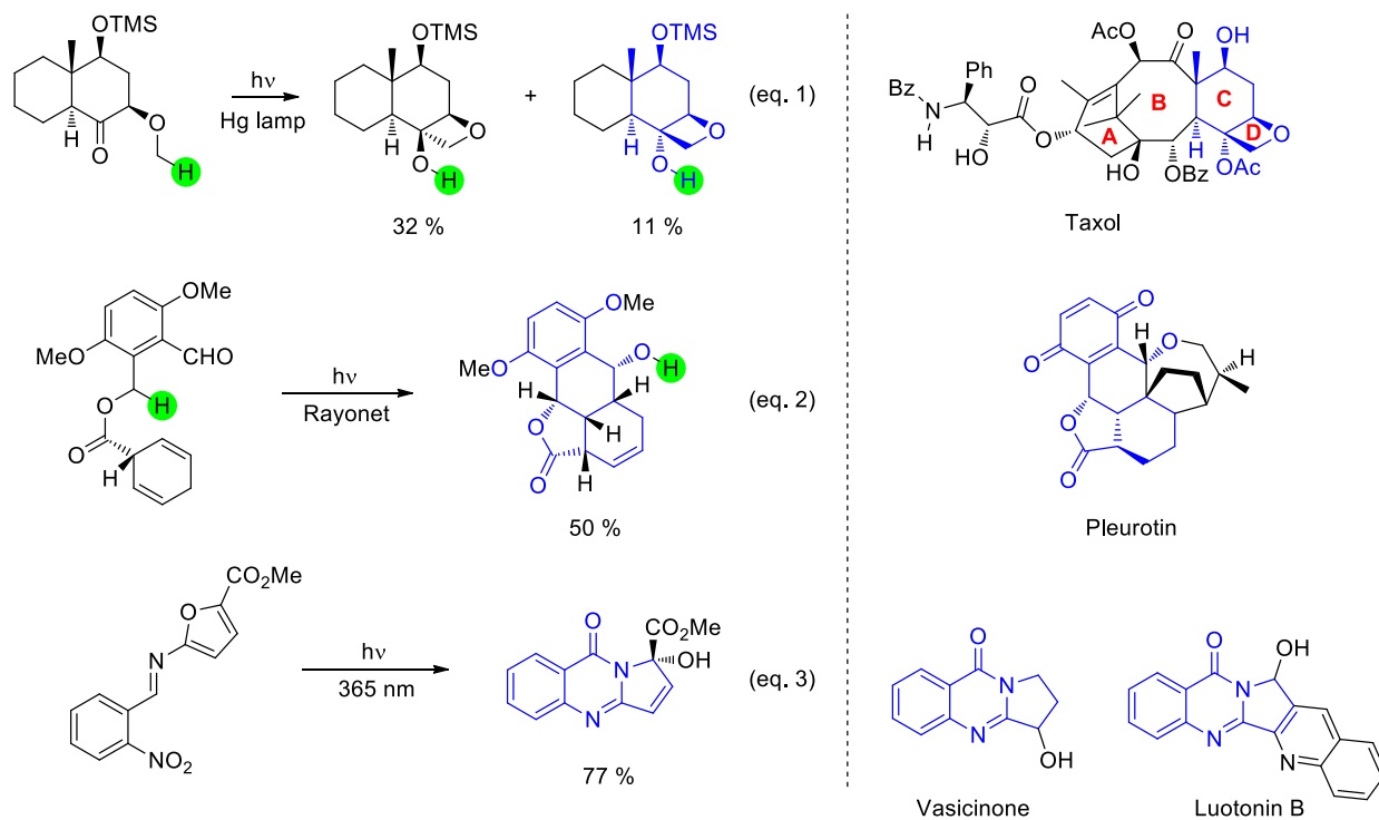
Scheme 11. – Synthesis of precursors of natural products Taxol, Pleurotin, Vasicinone and Luotonin B.
