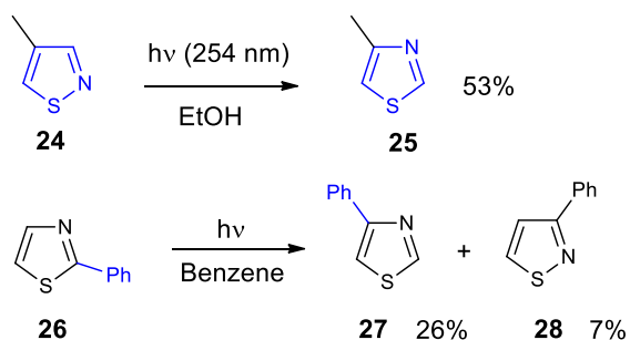
Scheme 5. Rearrangement of heteroatoms and migration of a substituent in isothiazole and thiazol derivatives.
