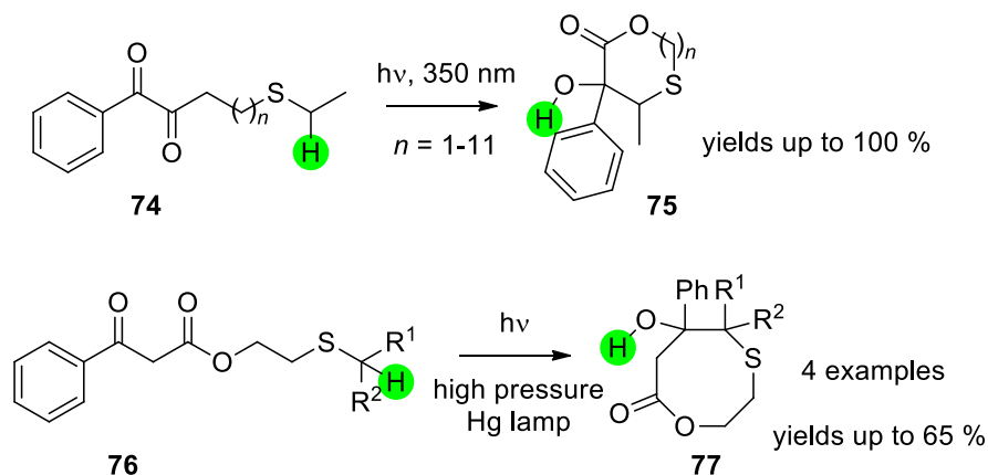
Scheme 17. Macrocyclization with thioether derivatives via hydrogen atom transfer.
