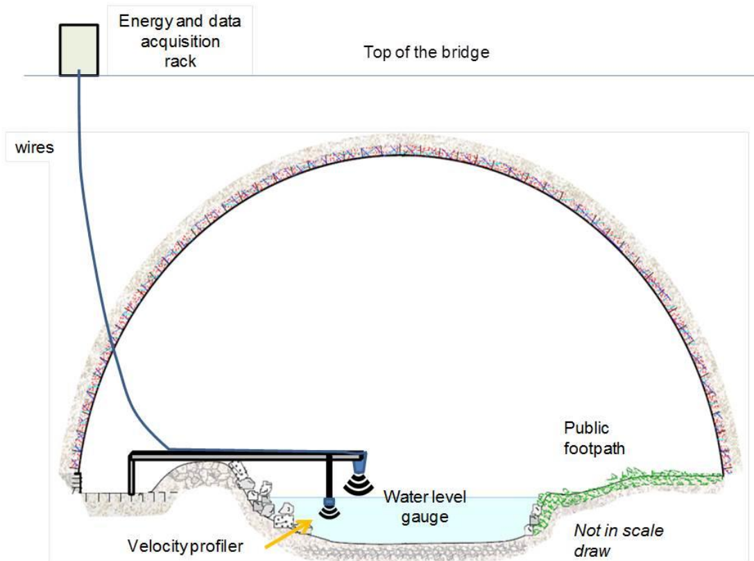
Figure 4 : Instrumentation scheme
