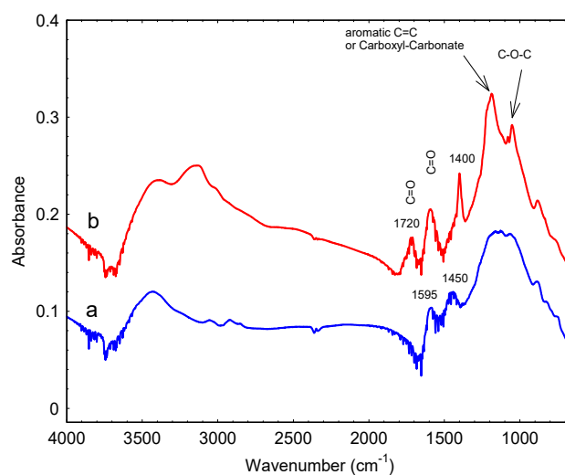
Figure 4. FTIR spectra of (a) hierarchical carbon beads and (b) activated hierarchical carbon beads after activation with APS.
