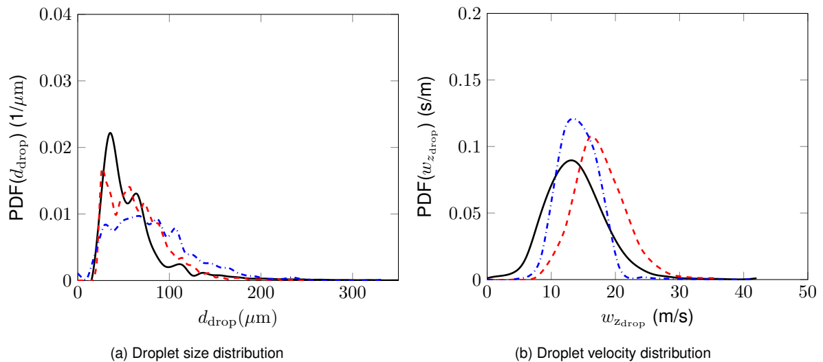
Figure 4. Characterization of droplets: Experiments (—), CLSVOF (---), and CLSMOF (-.-.-).
