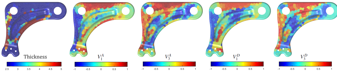
Figure 8: Step1. Optimal design variables distributions.
