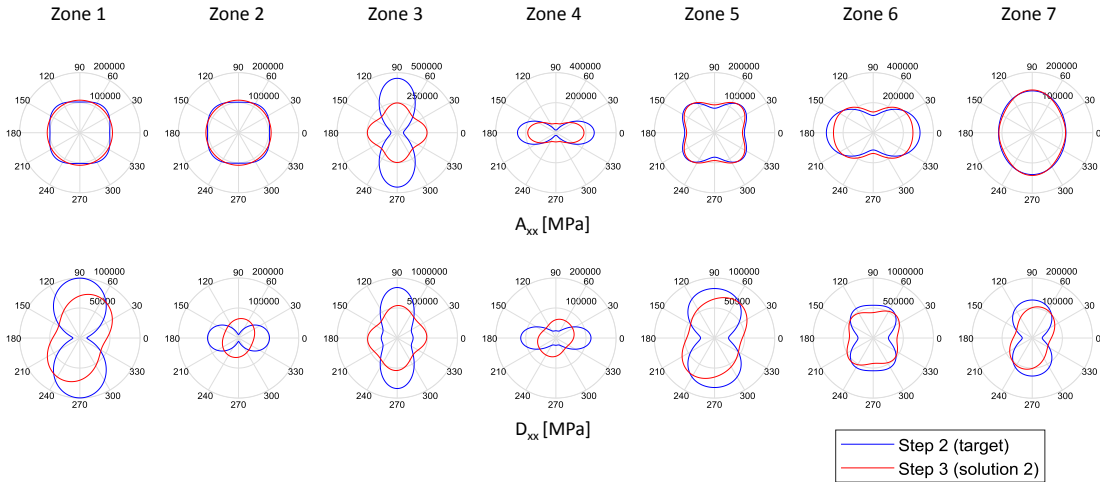
Figure 11: Step3. Solution 2. Stiffness matching with balanced laminates. Prescribed ( 0^\circ/90^\circ ) pair of plies on the bottom surface of the part and a ( \pm 45^\circ ) pair of plies on the top surface. Allowed ply orientations are 0^\circ, \pm 45^\circ, 90^\circ .
