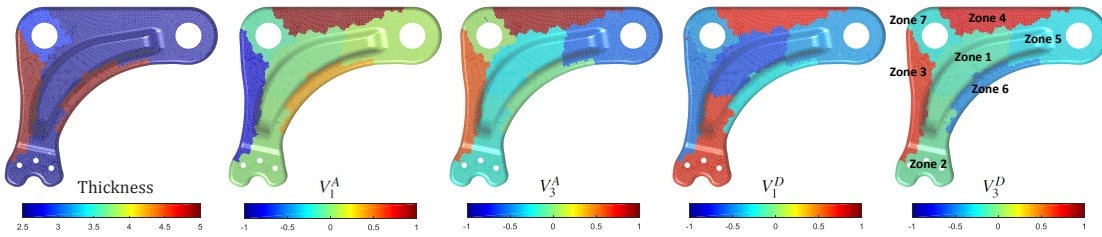
Figure 9: Step2. Optimal design variables distributions.
