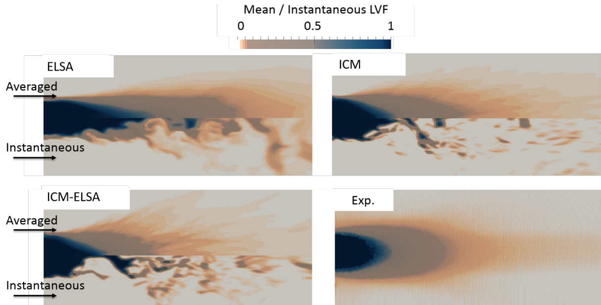
Figure 3. Mean (top half of each image) and instantaneous (bottom half of each image) values of Liquid Volume Fraction (LVF) fields of ELSA [24], ICM, ICM-ELSA. Mean LVF of experiments (bottom-right of the figure).
