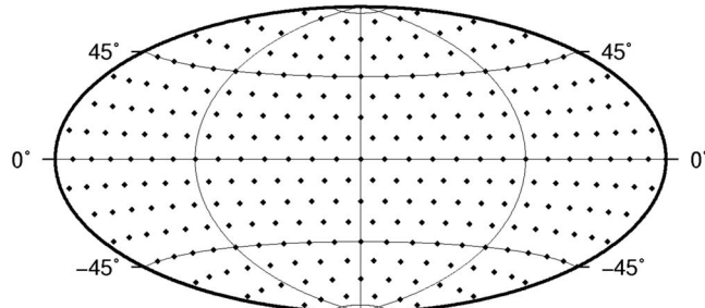
Figure 2. Example of a dipole mesh using the polar coordinate subdivision method for a dipole mesh parameter n_d = 15 .
