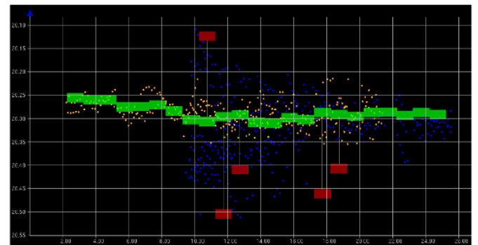
Fig. 6: Superimposition of CUBE hypothesis (in green: CUBE selected hypothesis in red: CUBE alternative hypothesis) to soundings within a slicing box (2D display from CARIS/HIPS software)
