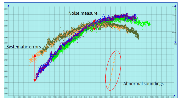
Fig. 2: Soundings within a slicing box colored by survey lines
