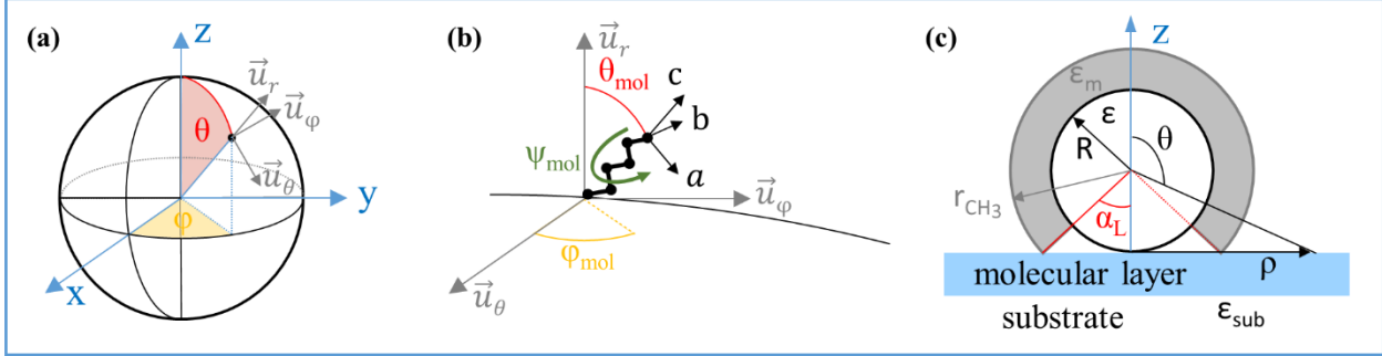
Figure 1 : Definitions of the three frames involved: (a) laboratory ( x,y,z ) and spherical ( u_\theta, u_\phi, u_r ); (b) molecular ( a,b,c ); (c) Sketch of the samples in the limit angle ( \alpha_L ) configuration. Molecules in the grey zone are considered in Part II whereas Part III deals with molecules in the blue zone.
