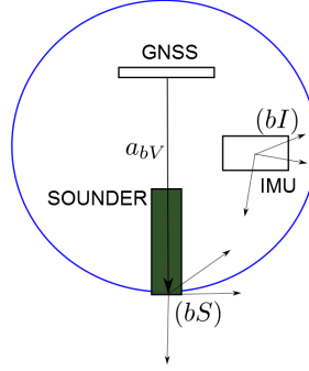
Fig. 3 HydroBall Sketch. The lever-arm vector a_{bV} is defined from the GNSS antenna center of phase to the SBES transducer acoustic center.
