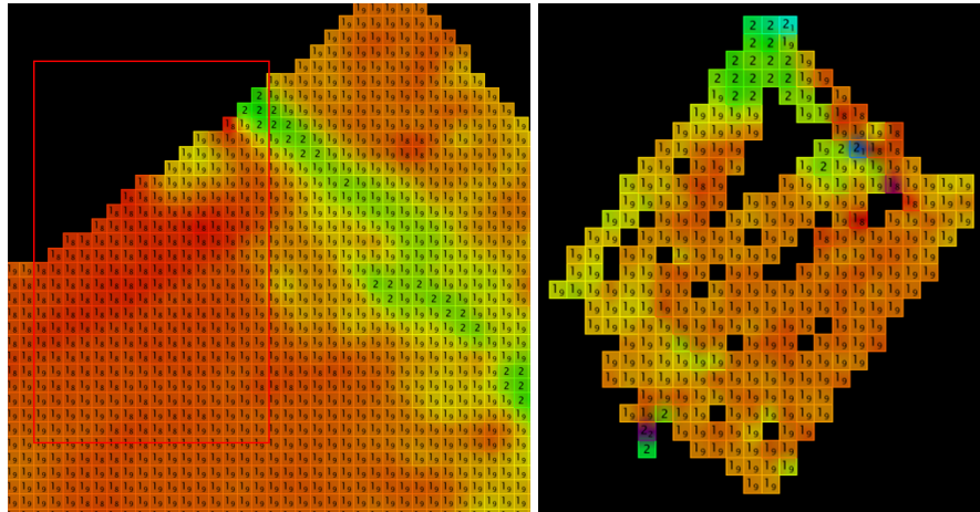
Fig. 6 MBES reference surface and Hydroball data (on the right). The red box shows the location of the overlap between HydoBall and MBES datasets.
