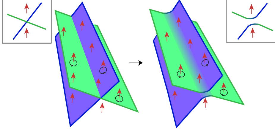
FIGURE 1. Given two surfaces S^{(1)}, S^{(2)} transverse to a vector field X , one considers the link \Gamma = \partial S^{(1)} \cup \partial S^{(2)} and blows up each of its components. In the resulting manifold M_\Gamma , the two surfaces (S^{(1)}, \partial S^{(1)}) and (S^{(2)}, \partial S^{(2)}) are surfaces with boundary whose intersection consists of circles and arcs ending on \partial M_\Gamma . The Fried sum (S^{(1)}, \partial S^{(1)}) \cup^F (S^{(2)}, \partial S^{(2)}) is then obtained by desingularizing these circles and arcs. In particular in the boundary \partial M_\Gamma \simeq \Gamma \times \mathbb{S}^1 , the boundaries \partial S^{(1)} and \partial S^{(2)} are circles transverse to X_\Gamma and to each other, and the desingularization is the unique reconnection of these circles that preserves transversality to X_\Gamma .
