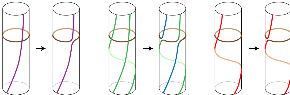
FIGURE 5. The Fried sum of the boundaries \partial\mathbb{T}_{2/3}^2 and \partial\mathbb{P} on the three components of \partial\mathbb{T}_{RW,\Gamma}^3 . One sees that \mathbb{T}_{2/3}^2 \overset{F}{\cup} \mathbb{P} has two boundary components along \gamma_O , and so four boundary components in total.
