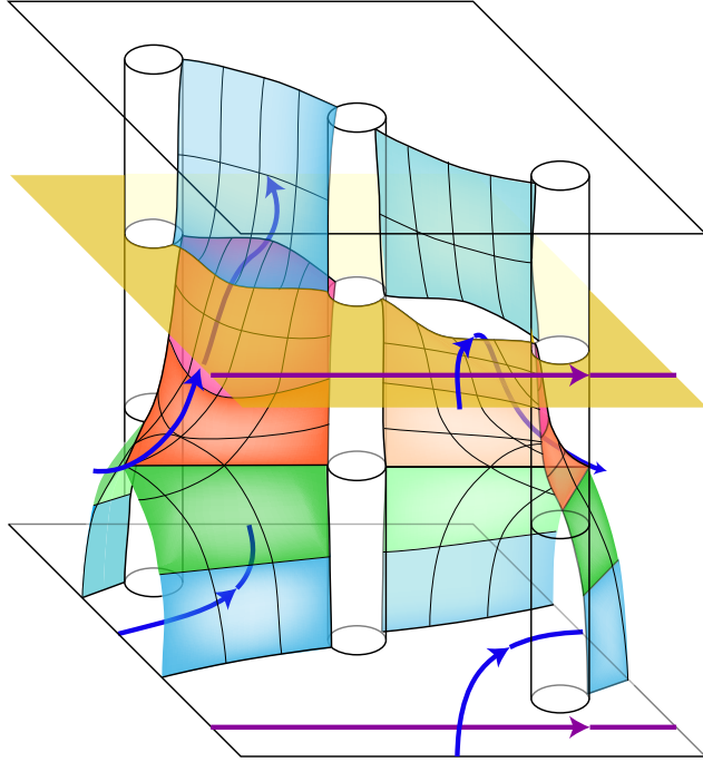
FIGURE 6. The desingularized sum \mathbb{T}_{2/3}^2 \overset{F}{\cup} \mathbb{P} in the 3-manifold \mathbb{T}_{RW,\Gamma}^3 . Also the curves \alpha' \times \{0\} and \beta' \times \{0\} and their images when pushed toward \mathbb{T}_{2/3}^2 \overset{F}{\cup} \mathbb{P} along \varphi_{\text{sus}} .
