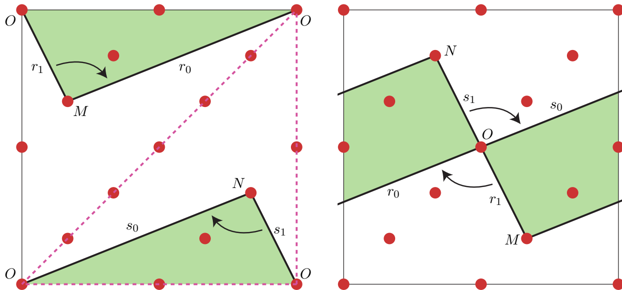
FIGURE 3. The parallelogram P_{RW} (green) in the torus \mathbb{T}^2 , here seen as the square [0, 1]^2 on the left, and as the square [-1/2, 1/2]^2 on the right. The red dots denote the fixed points of W . The segment r_1 is sent by W on r_0 , and s_1 is sent on s_0 . If W is not of the form R^m L^n or L^n R^m , then the point N lies in the interior of the dotted triangle, otherwise it lies on the vertical or diagonal border of this triangle.
