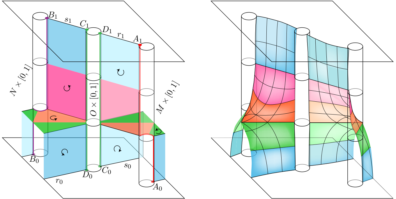
FIGURE 4. The ready-made \mathbb{P}^\perp and the tailored \mathbb{P} in \mathbb{T}_{RW,\Gamma}^3 , the 3-manifold obtained from \mathbb{T}_{RW}^3 by blowing-up the three periodic orbits O \times [0, 1] , M \times [0, 1] , and N \times [0, 1] . The map RW identifies the segments r_1 \times \{1\} with r_0 \times \{0\} , s_1 \times \{1\} with s_0 \times \{0\} , the points A_1 \times \{1\} with A_0 \times \{0\} , etc. One sees that \mathbb{P}^\perp and \mathbb{P} indeed have three boundary components : O \times [0, 1] along which \mathbb{P}^\perp wraps twice (in green), M \times [0, 1] minus once (in red), and N \times [0, 1] minus once (in purple).
