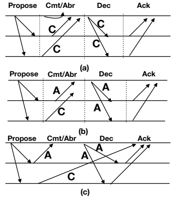
Fig. 2. Two-phase-commit: (a) and (b) are lock-step executions, (c) is a runtime execution.
