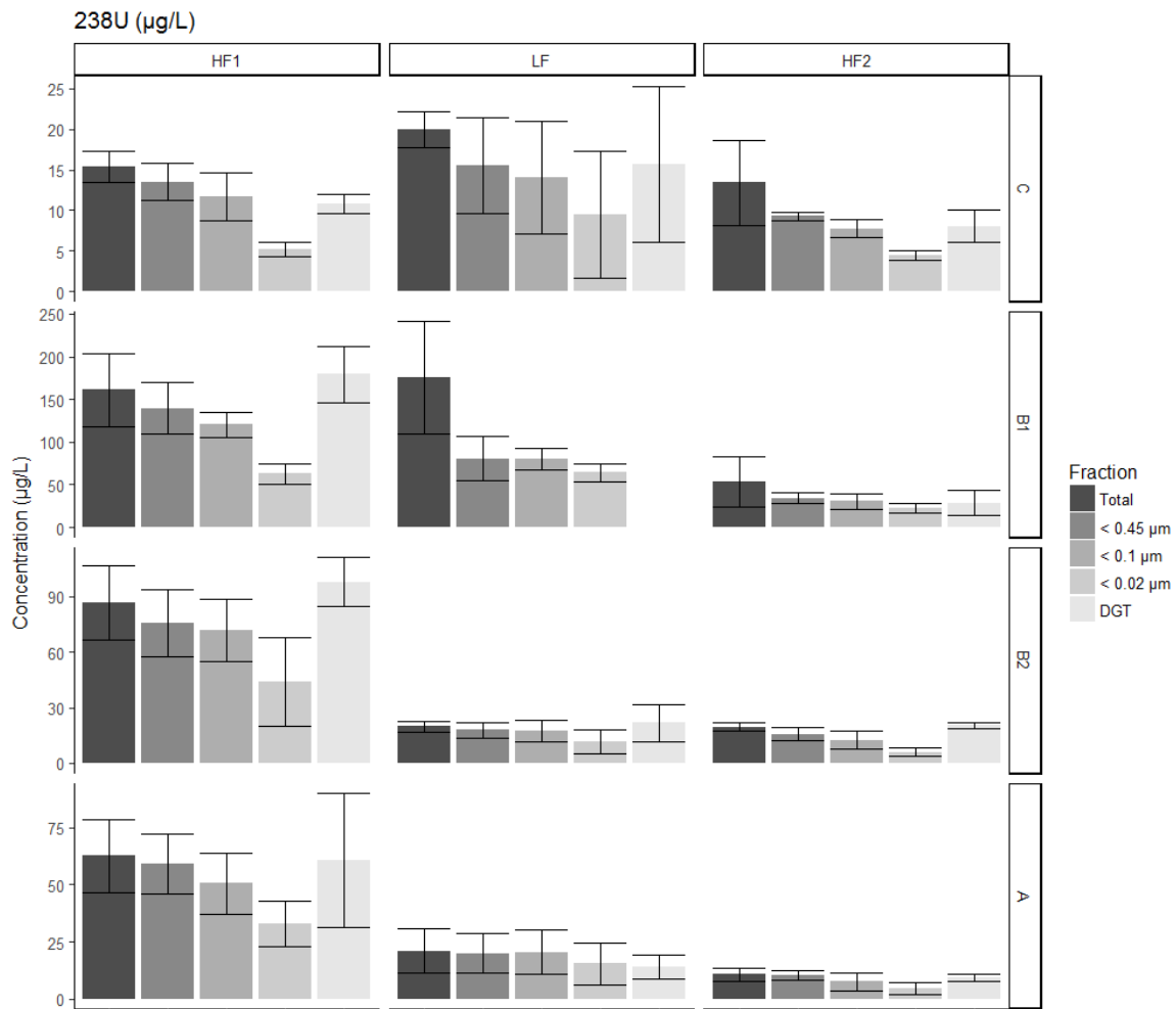
487 Figure 6: Concentrations of uranium in raw, 0.45 \mu\text{m} , 0.1 \mu\text{m} and 0.02 \mu\text{m} filtered water samples 488 and DGT-labile concentrations over the three monitoring periods 489 (period variability expressed as a standard deviation)
