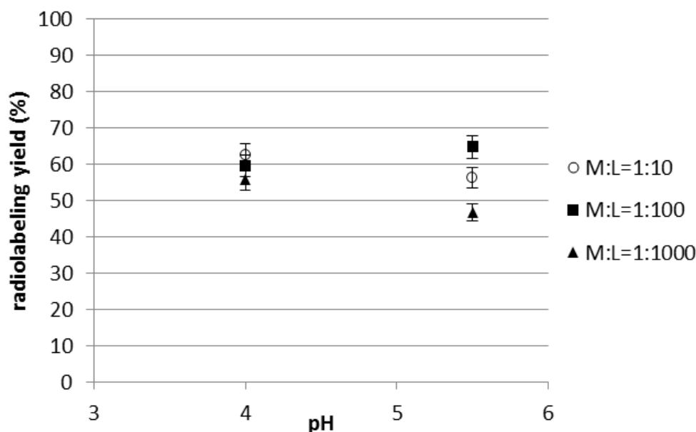
Figure 4: Evolution of the radiolabeling yields for AGuIX@DOTA2% as a function of pH for 44 Sc.
