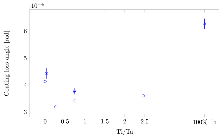
Figure 5. Mechanical loss of annealed Ta 2 O 5 -TiO 2 films deposited with the GC, as a function of the mixing ratio Ti/Ta; the data point of poly-crystalline TiO 2 is also shown, for comparison. For clarity, only values measured at ~ 2.5 kHz are shown; the same trend has been observed at ~ 10 kHz.
