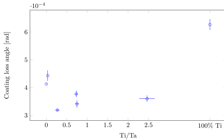
Figure 5. Mechanical loss of annealed \text{Ta}_2\text{O}_5\text{-TiO}_2 films deposited with the GC, as a function of the mixing ratio \text{Ti}/\text{Ta} ; the data point of poly-crystalline \text{TiO}_2 is also shown, for comparison. For clarity, only values measured at \sim 2.5 kHz are shown; the same trend has been observed at \sim 10 kHz.
