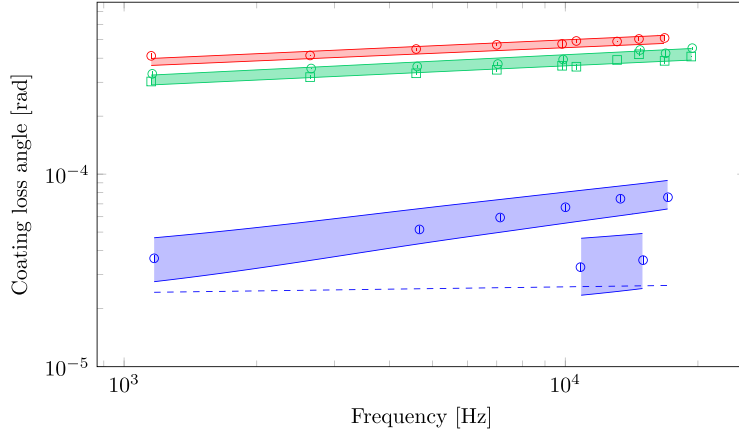
Figure 2. Mechanical loss of coating materials of Advanced LIGO, Advanced Virgo and KAGRA after annealing: Ta 2 O 5 (red), Ta 2 O 5 -TiO 2 (green), SiO 2 (blue). Different markers denote distinct samples; error bars are shown, though barely visible. Shaded regions represent uncertainties from fitting a frequency-dependent loss model to each data set: \phi_c(f) = af^b via least-squares linear regression for Ta 2 O 5 and Ta 2 O 5 -TiO 2 , \phi_c(f) = af^b + \epsilon d\phi_e via numerical non-linear regression for SiO 2 ; the dashed curve shows the behavior of the af^b term only for SiO 2 .
