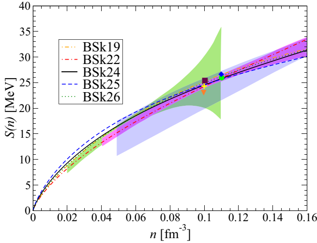
FIG. 2. Variation of the symmetry energy S(n) at subsaturation densities n for the functionals BSk19, BSk20, BSk21, BSk22, BSk24, BSk25, and BSk26. The shaded areas are experimental constraints: from heavy-ion collisions [56] (blue), from isobaric-analog states and neutron skins [57] (purple), and from the electric dipole polarizability of ^{208}\text{Pb} [58] (green). Symbols are values inferred from doubly magic nuclei [59] (square), Fermi-energy difference [60] (circle), binding-energy differences among heavy isotope pairs [61] (diamond), giant dipole resonance in ^{208}\text{Pb} [62] (cross), giant quadrupole resonance in ^{208}\text{Pb} [63] (triangle). Results for BSk20 and BSk21 are indistinguishable from those obtained for BSk26 and BSk24, respectively.
