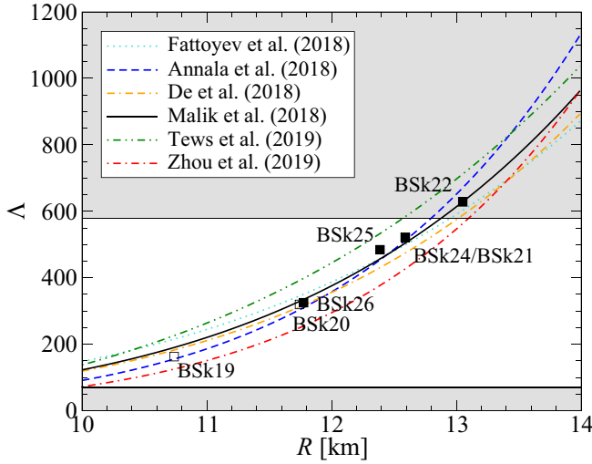
FIG. 4. Tidal deformability coefficient \Lambda of a 1.4 M_{\odot} NS as a function of the radius R , as predicted by selected empirical relations proposed by various authors (lines). For comparison, results obtained using the unified EoSs considered in this work are also shown (symbols). The central area represents the LIGO-Virgo constraint \Lambda = 190^{+390}_{-120} at 90% confidence level using method (ii) [11]. See text for details.
