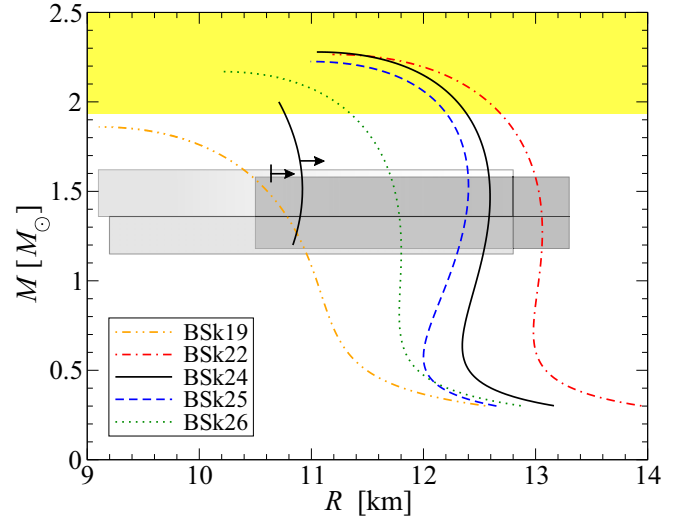
FIG. 6. Gravitational mass M (in solar masses) versus circumferential radius R of nonrotating NSs, calculated using the unified EoSs of Refs. [33,34]. Results for BSk20 and BSk21 are indistinguishable from those obtained for BSk26 and BSk24, respectively. Constraints inferred from the analysis of GW170817 are also shown: lines with arrows are lower bounds on the radius from Refs. [84,85]; dark and light boxes are the masses and radii of the two NSs (90% confidence level) as inferred by the LIGO-Virgo collaboration using method (iii) with the additional requirement M_{\text{max}} = 1.97 M_\odot , and (ii) respectively; the yellow area denotes expected values for the maximum mass as obtained by various studies. See text for details.
