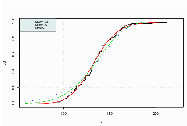
Figure 10: Plots of the estimated cdfs.
