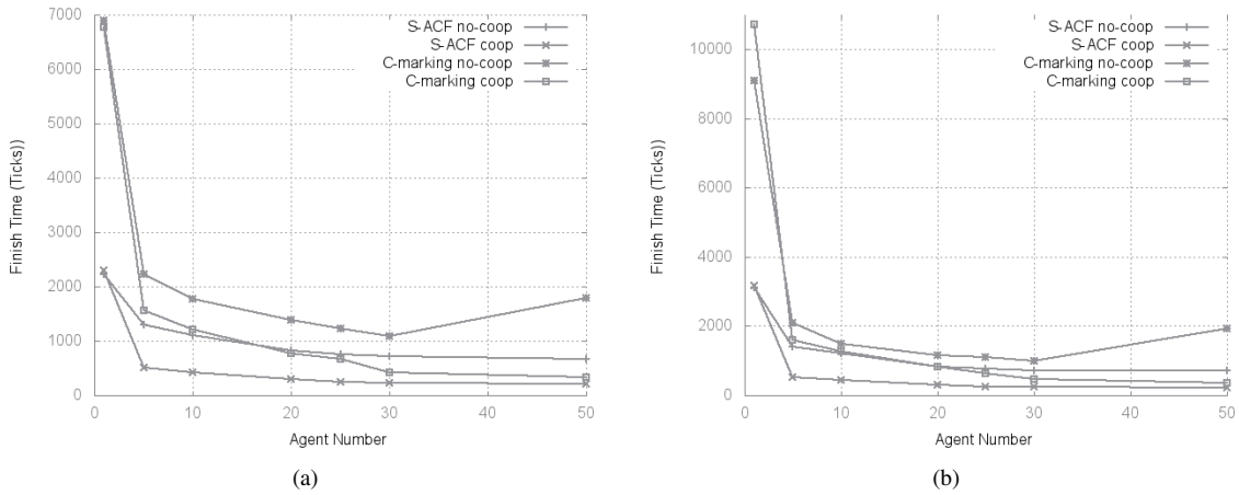
Fig. 4: Comparison results of S-ACF no-coop, S-ACF coop, C-marking no-coop and C-marking coop, when varying the agent number (a) Obstacle-free environment (b) Obstacle environment
