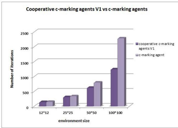
Fig. 4. Results comparison with c-marking agents model
