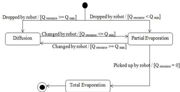
Fig. 1. State diagram of our digital pheromone
