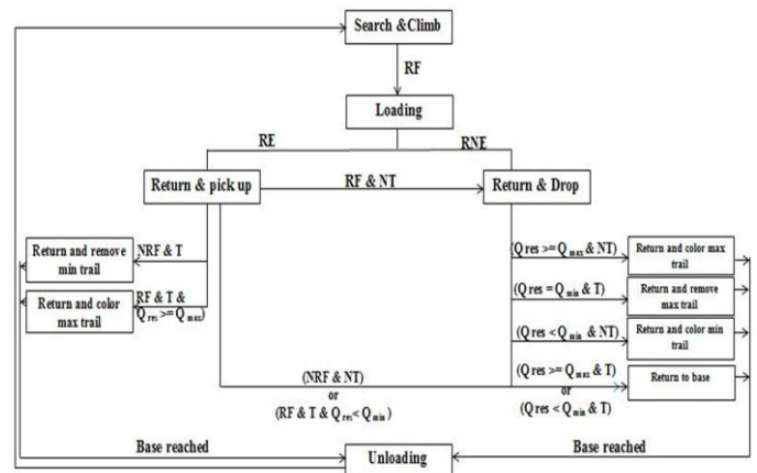
Fig. 2. State diagram of our digital pheromone
