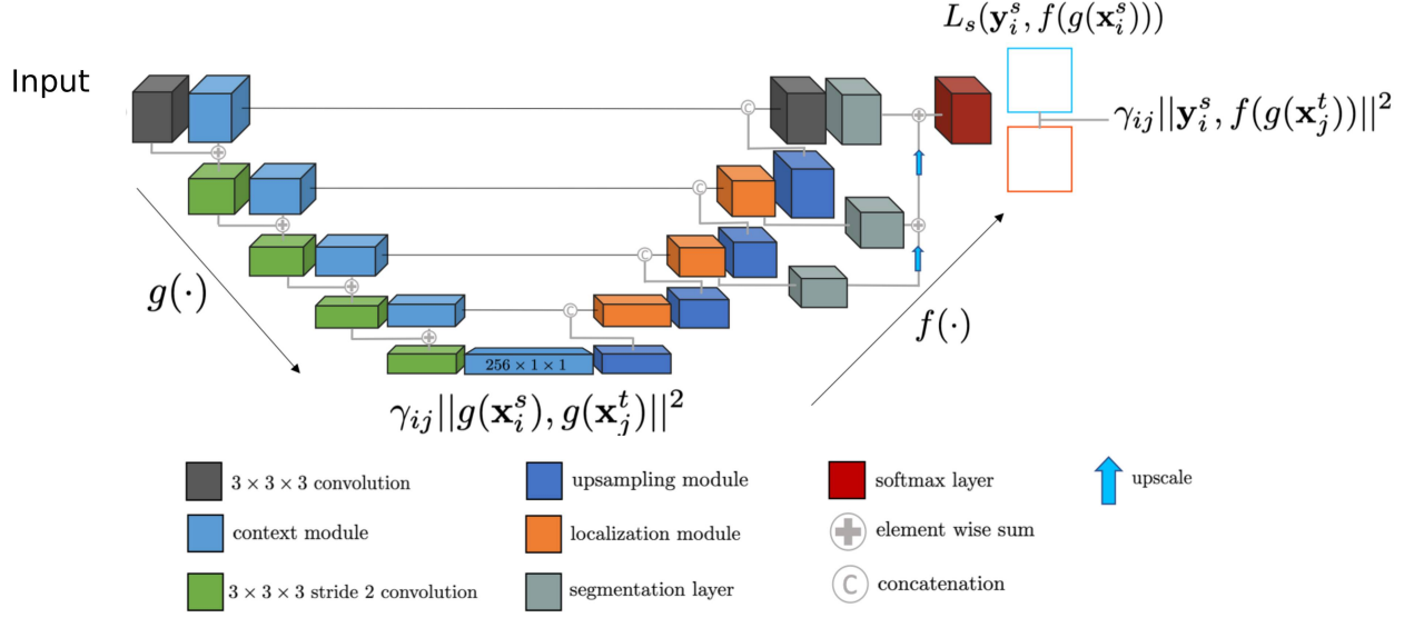
Figure 1: The Seg-JDOT framework. g(\cdot) is the embedding function, f(\cdot) is the segmenter and, in between them, the bottleneck representation is the latent space \mathbf{z} where we perform the adaptation. We report the terms of the Equation 8 at the levels where they are applied. We represent the output source images with a blue square and the output target images with a red square.
