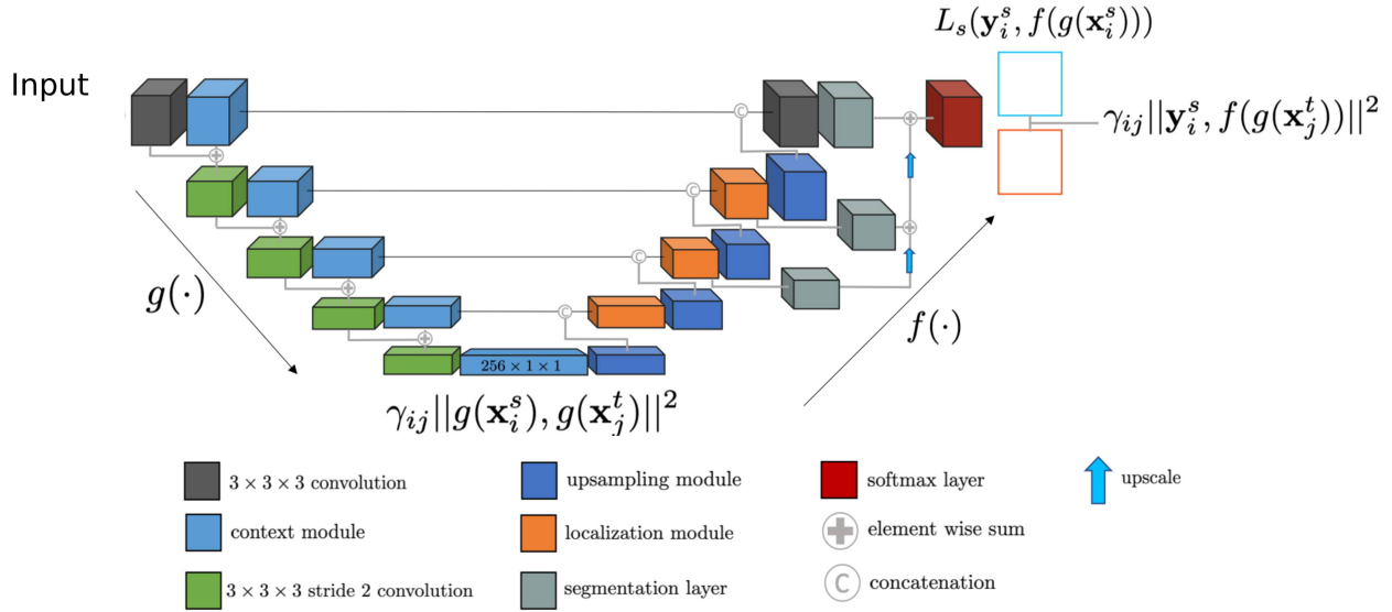
Figure 1: The Seg-JDOT framework. g(\cdot) is the embedding function, f(\cdot) is the segmenter and, in between them, the bottleneck representation is the latent space \mathbf{z} where we perform the adaptation. We report the terms of the Equation 8 at the levels where they are applied. We represent the output source images with a blue square and the output target images with a red square.
