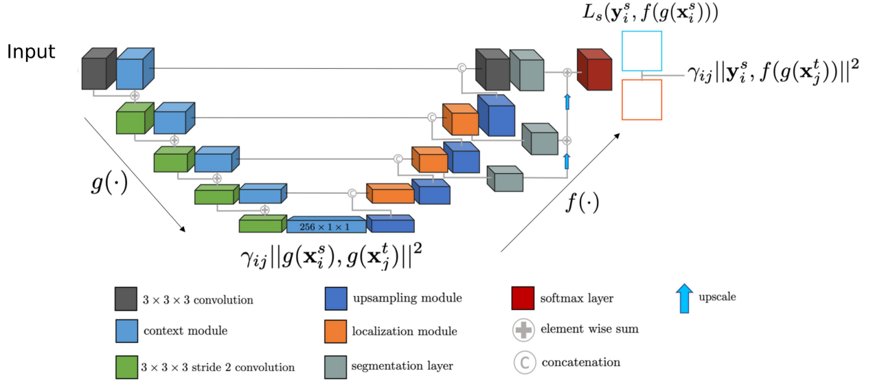
Figure 1: The Seg-JDOT framework. g(\cdot) is the embedding function, f(\cdot) is the segmenter and, in between them, the bottleneck representation is the latent space z where we perform the adaptation. We report the terms of the Equation 8 at the levels where they are applied. We represent the output source images with a blue square and the output target images with a red square.
