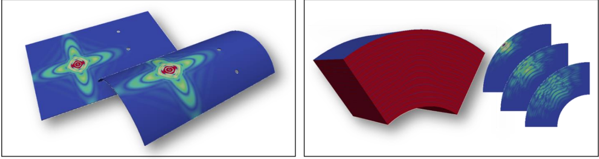
FIGURE 3. Simulation of guided (left) and bulk (right) wave propagation in curved stratified composites.
