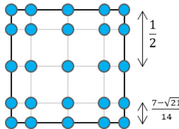
FIGURE 4. 4 th order Gauss-Lobatto points on the unit quadrilateral.
