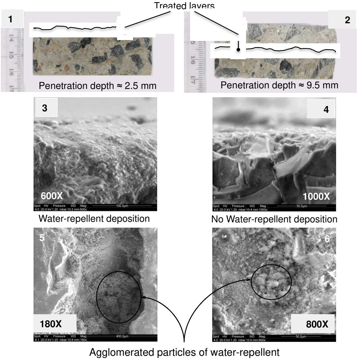
199 Figure 3: Multi-scan approach of water repellents penetration (image 1 and 2: 200 transversal sections, images 3 and 4: SEM scans of concretes surface, images 5 201 and 6: SEM scans of the pores surface
