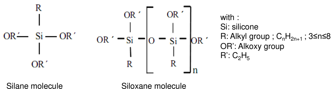
Figure 1: Silane and siloxane molecule [Johansson, 2010]
