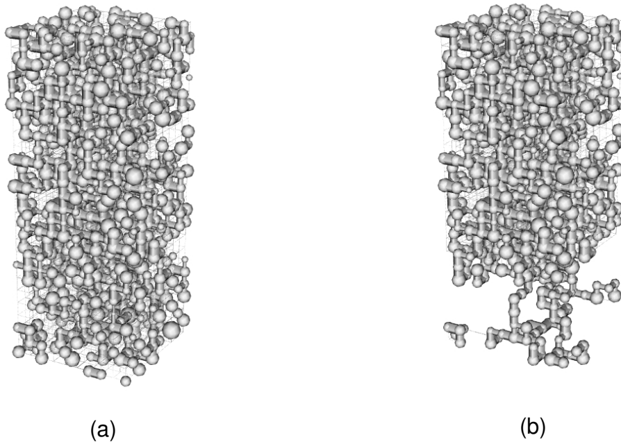
Figure 8: A realization of a 10 \times 25 \times 10 pore network before (a) and after (b) removing small pores in a layer of thickness equal to 30% of the total height of the network.
