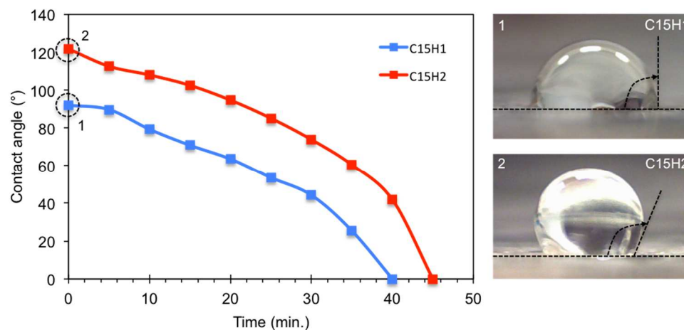
Figure 6: Contact angle as a function of time and water repellents used (H1 and H2) on C15 concrete
