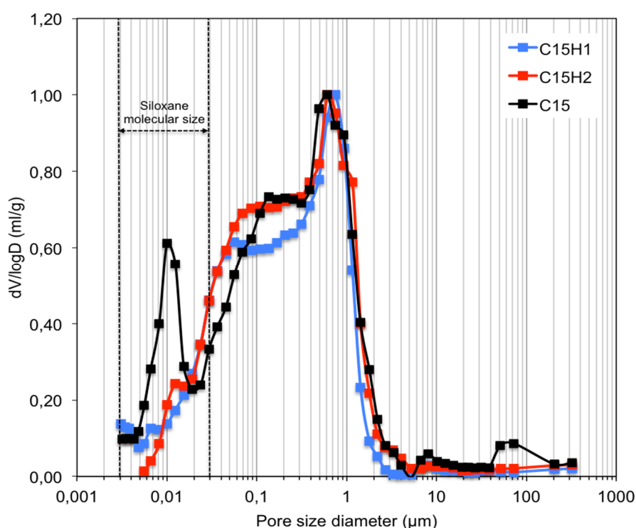
Figure 4: Pores size distribution of C15, C15H1 and C15H2 concretes
