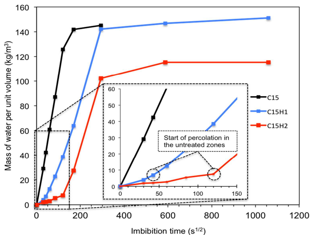
Figure 5: Capillary absorption of C15, C15H1 and C15H2 concretes
