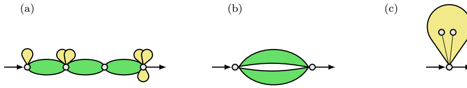
Fig. 7: The three main cases for extracting a term from a K_4 -free graph.
