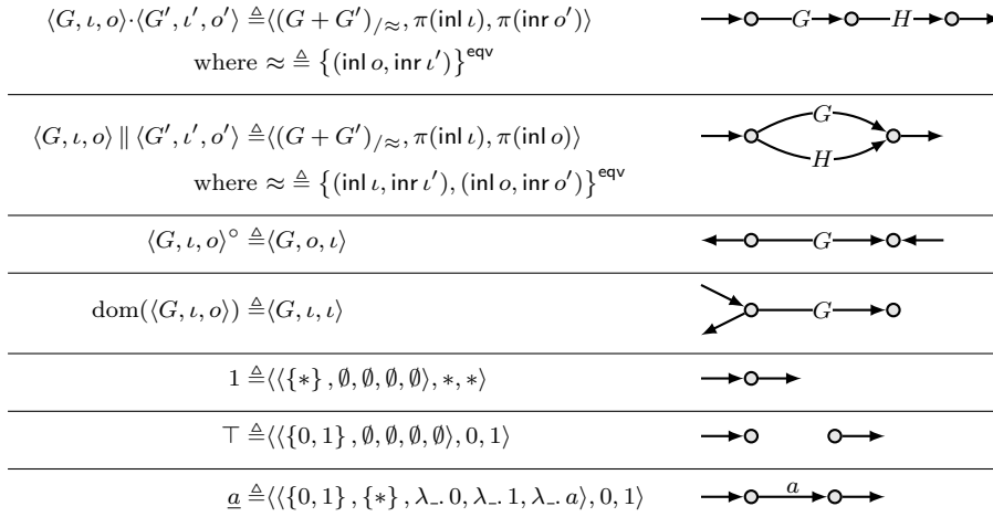
Fig. 6: The algebra of 2p-graphs.
