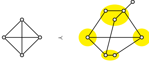
Fig. 3: Exhibiting K_4 as a minor
