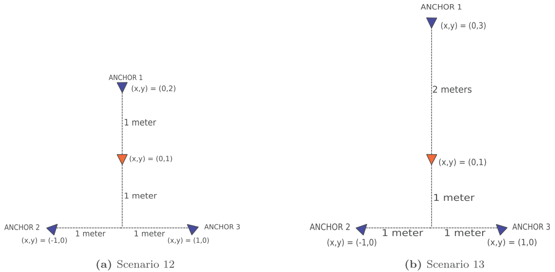
Fig. 22. Scenario set-up.
