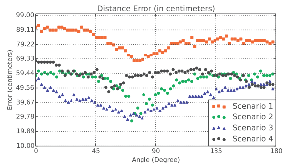
Fig. 16. Distance error versus angle of incidence (antenna).
