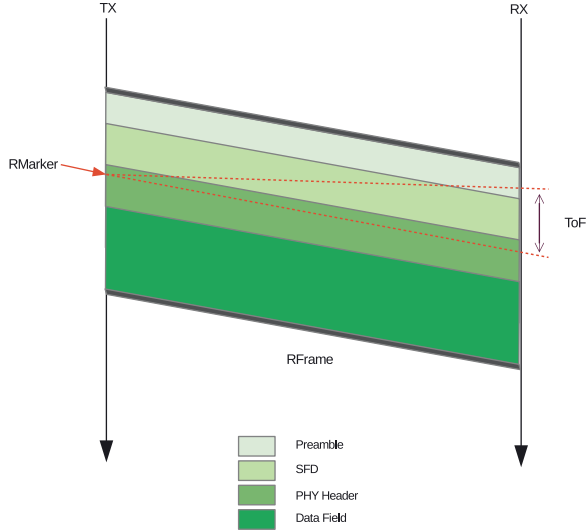
Fig. 6. Ranging support in IEEE 802.15.4a packet.
