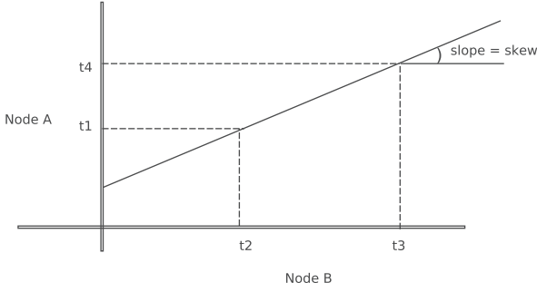
Fig. 7. Skew estimation.
