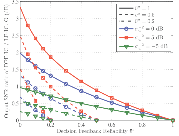
Fig. 5. Post-equalization SNR ratio G depending on channel SNR \sigma_w^{-2} , prior reliability \bar{v}^a and “decision” reliability \bar{v}^c .
