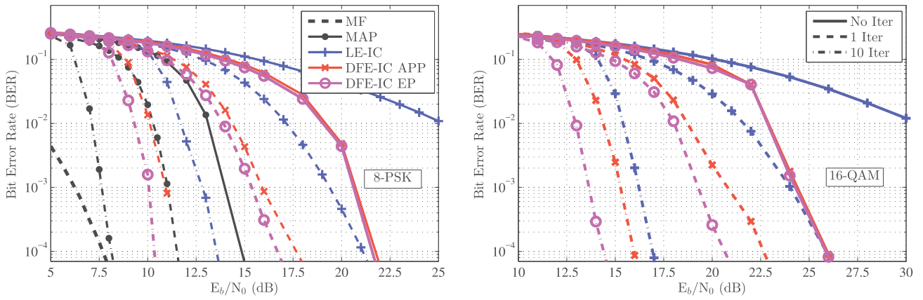
Fig. 9. BER performance of the proposed DFE-IC in Proakis-C with 8-PSK and 16-QAM constellations.
