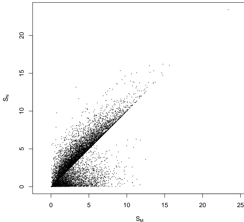
FIGURE 1. The figure shows 10^4 simulated pairs (A, B) , with \mu = \sum_{n=2}^5 \frac{1}{4}\delta_n and \nu = \frac{1}{4}\delta_1 + \frac{1}{4}\delta_3 + \sum_{n=4}^6 \frac{1}{6}\delta_n , \text{Law}(X_i) = \mathcal{E}(1) , and the algorithm of Section 2.3 to produce the diatomic decomposition.
