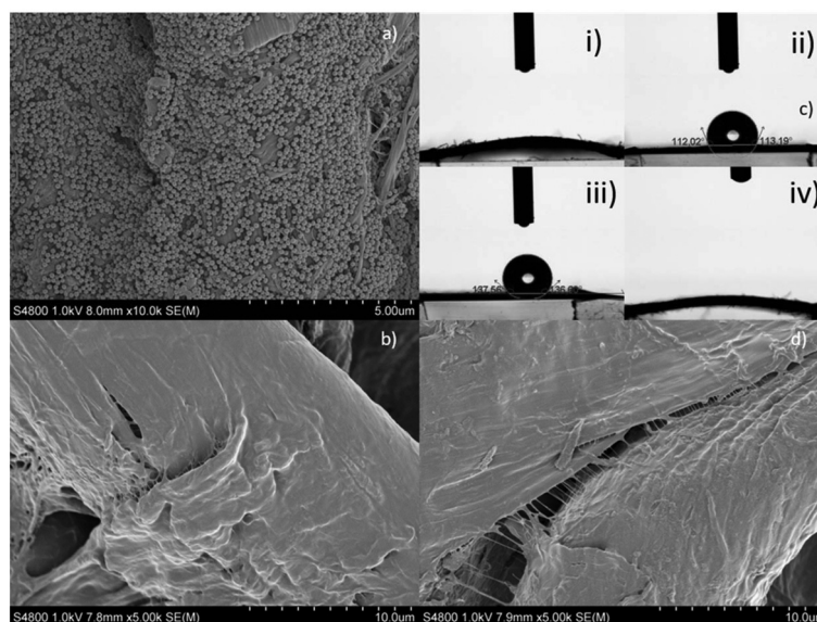
Fig. 7 SEM images of filter papers covered with latexes ( 0.1\text{ g L}^{-1} , 10 mM NaCl); (a) \text{PMMA}_{Tg120} , (b) \text{P(BA-co-MMA)}_{Tg3} , (c) water CA measurements prior to annealing (i) \text{PMMA}_{Tg120} (ii) \text{P(BA-co-MMA)}_{Tg3} and (iii) \text{PBA}_{Tg-40} . Inset (iv) filter paper with \text{PMMA}_{Tg120} after annealing at 140^\circ\text{C} for 3 h and (d) \text{PBA}_{Tg-40} .
