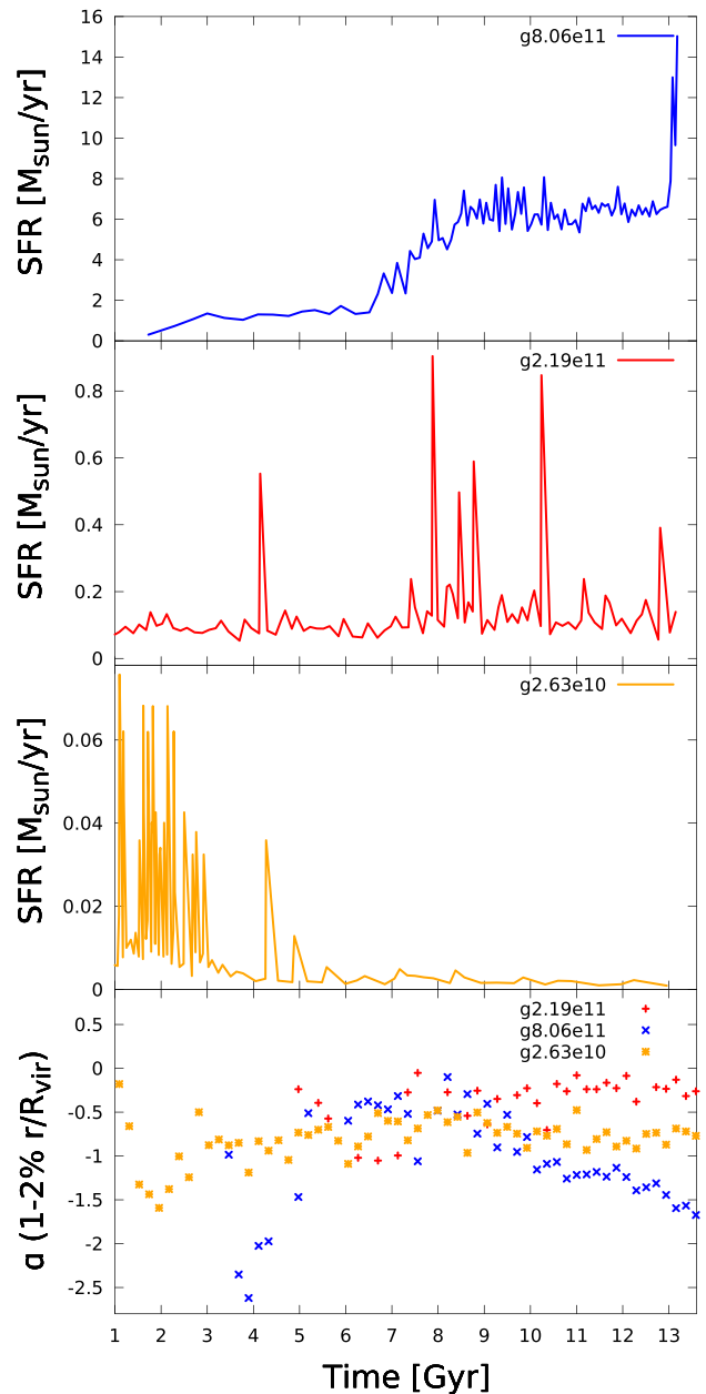
Figure 8. Time evolution of the star formation rate (SFR, upper panels) and the central density slope ( \alpha , lower panel), for our three test galaxies: g8.06e11 (blue), g2.19e11 (red) g2.63e10 (orange).
