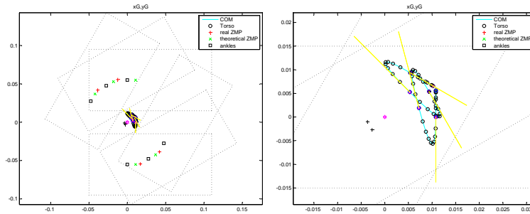
Fig. 2. Footprints with center of mass trajectory, theoretical and real zero moment points in rotation motion of 60[deg] about the middle of ankle joint centers. Model of linear inverted pendulum. The right view is a zoom of the COM trajectory from left view.
