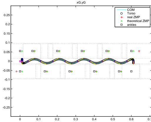
Fig. 1. Footprints with center of mass trajectory, theoretical and real zero moment points in forward motion of 0.6[m] . Model of linear inverted pendulum.
