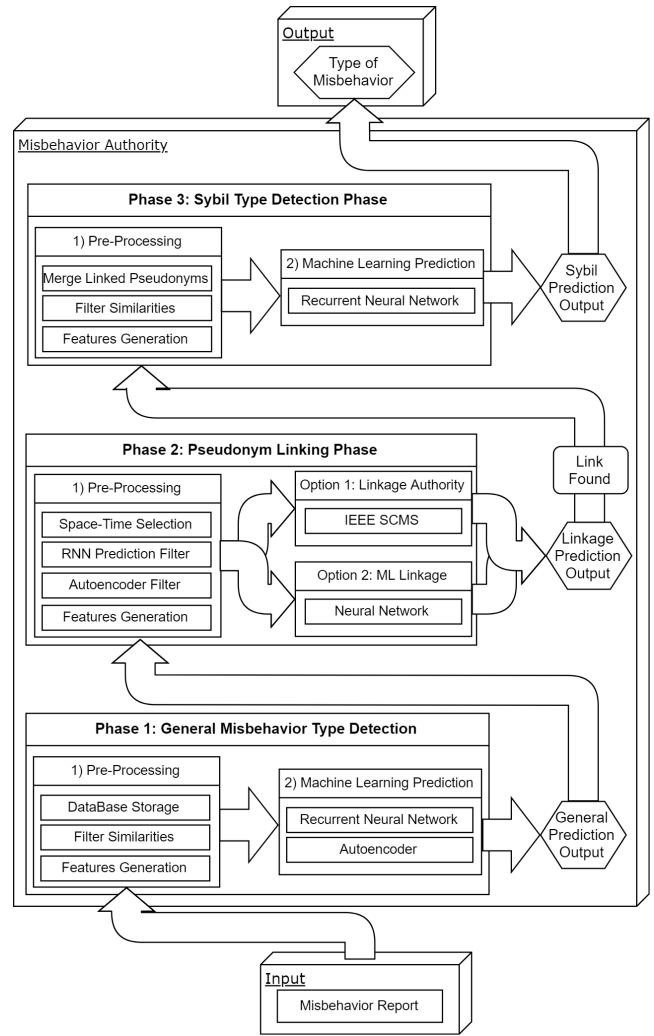
Fig. 6: Global Detection System Architecture
