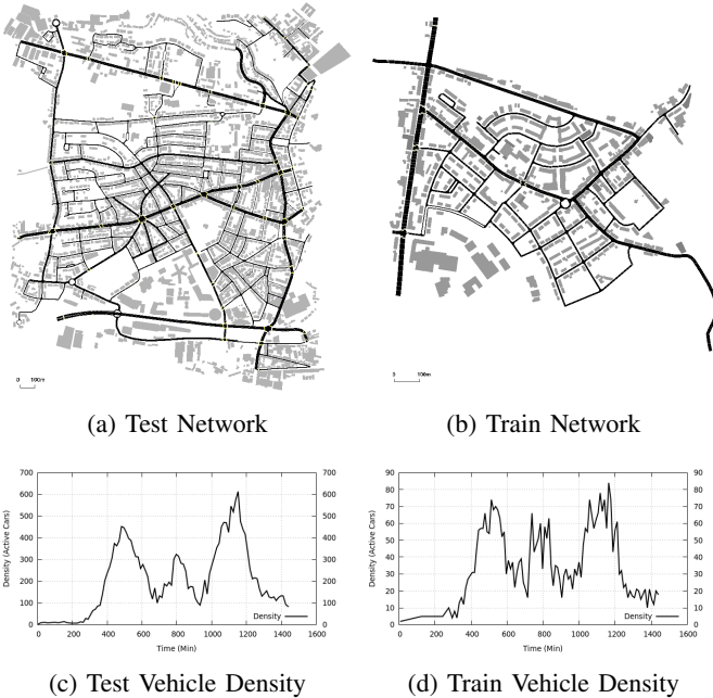
Fig. 7: Simulation Scenario: Part of Luxembourg city
