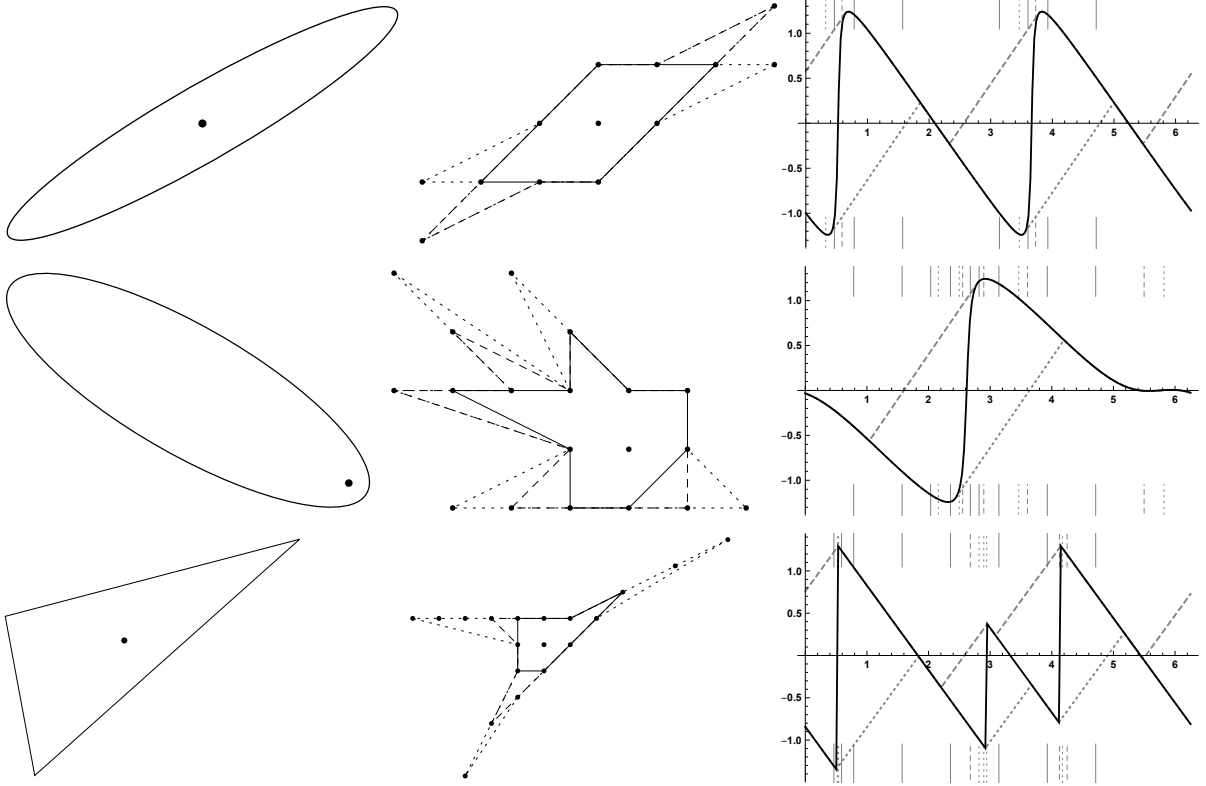
Figure 1: Left: Unit sphere \{F = 1\} of a norm F , which is asymmetric in the second and third row. The origin is marked with a point. Center: Minimal (F, \alpha) -acute stencil for \alpha = \pi/2 (solid), \pi/3 (dashed), \pi/4 (dotted). Right: Function \varphi_F (solid), \psi_F^+ (dashed, above), \psi_F^- (dotted, below). Vertical bars correspond to the angles of the stencil points.
