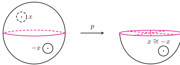
Fig. 3. The b^{2k+1} -symplectic structure on the sphere S^2 that vanishes at the equator induces a b^{2k+1} -symplectic structure on the projective space \mathbb{R}P^2 .
