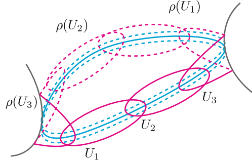
Fig. 4. A collar of compatible neighborhoods.
