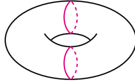
Fig. 2. Example: b^m -symplectic structure in the torus.
