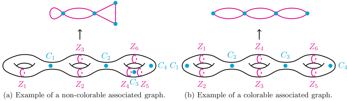
Fig. 5. Examples of associated graphs.
