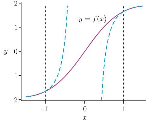
Fig. 1. Smooth and odd extension of f inside the interval [-1, 1] such that f' > 0 .
