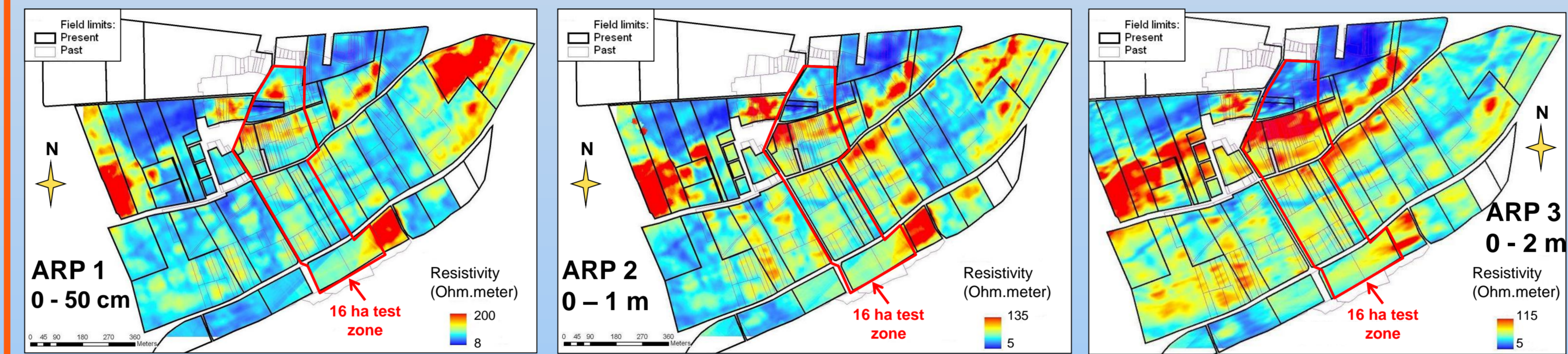
Fig. 3.1: Soil resistivity maps at 3 different depths of investigation
