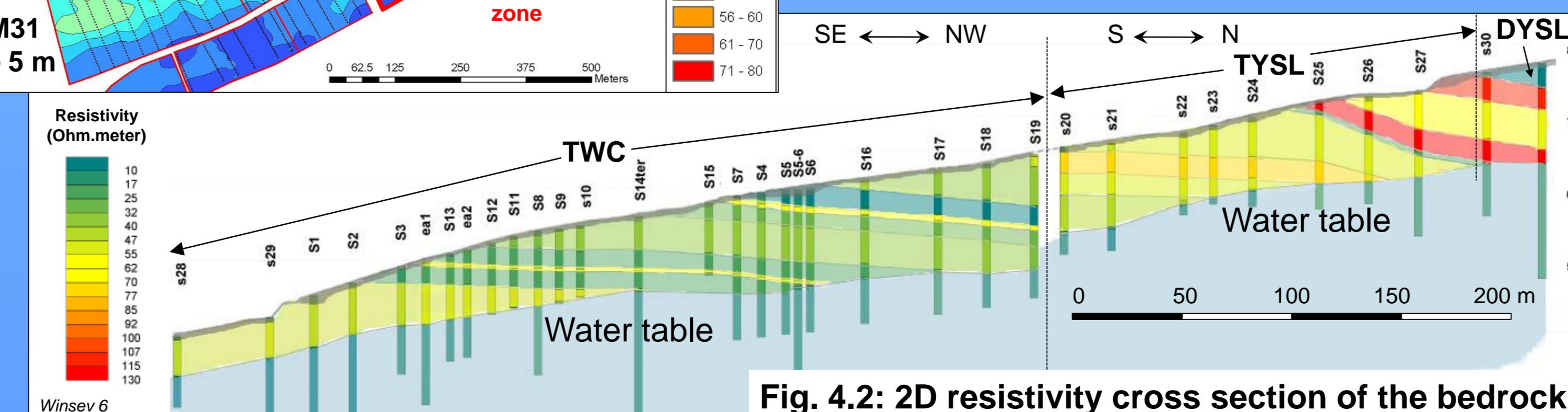
Fig. 4.2: 2D resistivity cross section of the bedrock
