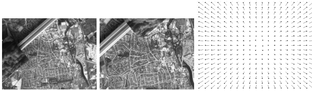
Fig. 7 First and last frames of the second robot sequence, and the dominant flow between frames 0 and 1 computed with TS model.
