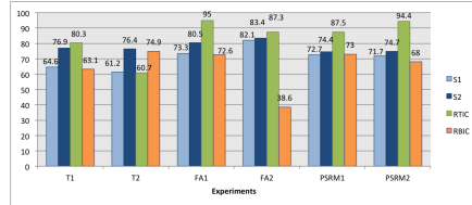
Fig. 4 Rates of correct classification for each group of experiments obtained with the four model selection criteria (given in percentage of the total number of examples in each experiment).
