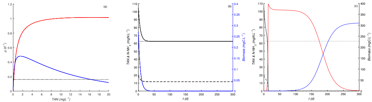
Figure 3. Simulation results obtained under a continuous supply with a high TAN concentration (dotted line in (b) & (c)) at a fixed dilution rate (dotted line in (a)). (a) growth functions previously identified for C. Sorokiniana (in solid red line) and S. pectinatus (in solid blue line), (b) dynamics when S. pectinatus is cultivated alone, (c) dynamics when S. pectinatus and C. Sorokiniana are cultivated together. In (b) and (c), the biomass variations over time are presented in blue for Scenedesmus sp. and in red for Chlorella sp. while the substrate variations are in solid black lines for TAN and in black dashed lines for NH_3 .
