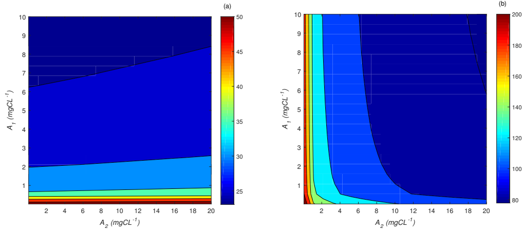
Figure 4. Isovalue diagrams: resilience time (a) and succession time (b) (in days) depending on the initial biomass densities of C. sorokiniana ( A_1 ) and S. pectinatus ( A_2 ) (in mgC.L^{-1} ) under a continuous supply of a high nitrogen concentration.
