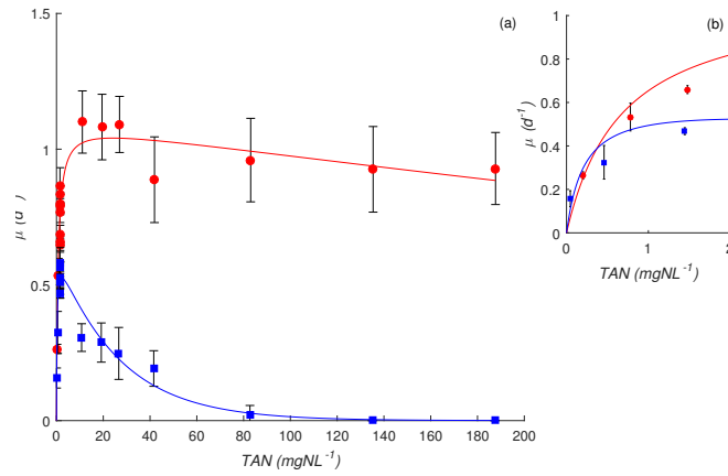
Figure 2. SE2 and SE3 data sets (full points) compared to the proposed kinetic model for C. sorokiniana (continuous red line) and S. pectinatus (continuous blue line) in (a), with a focus on low TAN concentrations in (b) (Data points are the mean of 3 duplicate measurements of growth rate).
