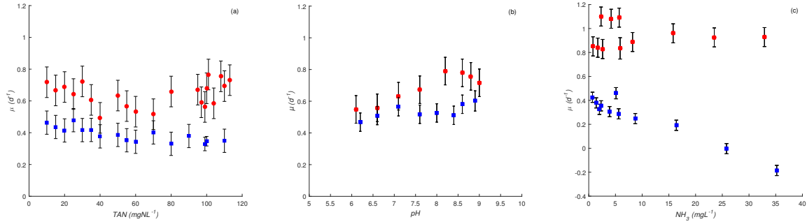
Figure 1. Growth rates from multiple comparisons of Matlab tests on growth rate values estimated based on ANCOVA analyses for C. sorokiniana (in red) and S. pectinatus (in blue) at different levels of (a) TAN concentrations, (b) pH conditions, (c) NH_3 concentrations.
