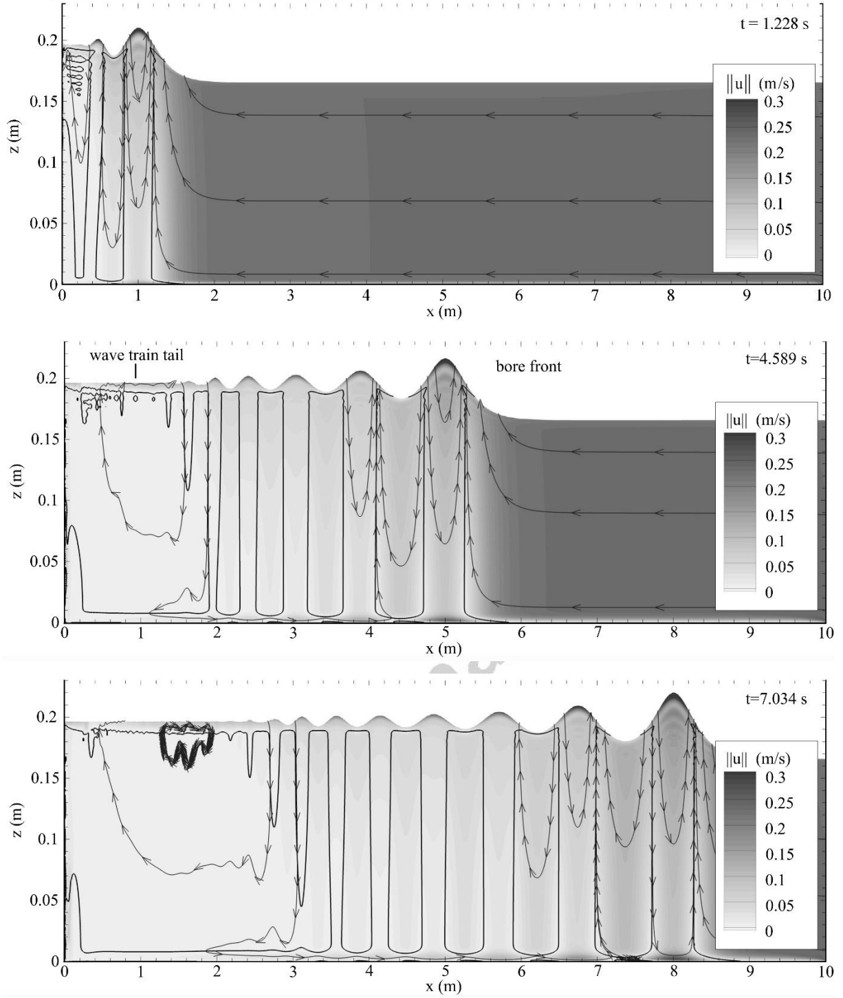
Fig. 4 Case A: dominated by undulations, mapping of the velocity magnitude \|u\| in the water during the bore propagation at 3 different times with velocity streamlines (lines with arrows) and the isoline u_x = 0 (black lines). Axis scales are independent.
