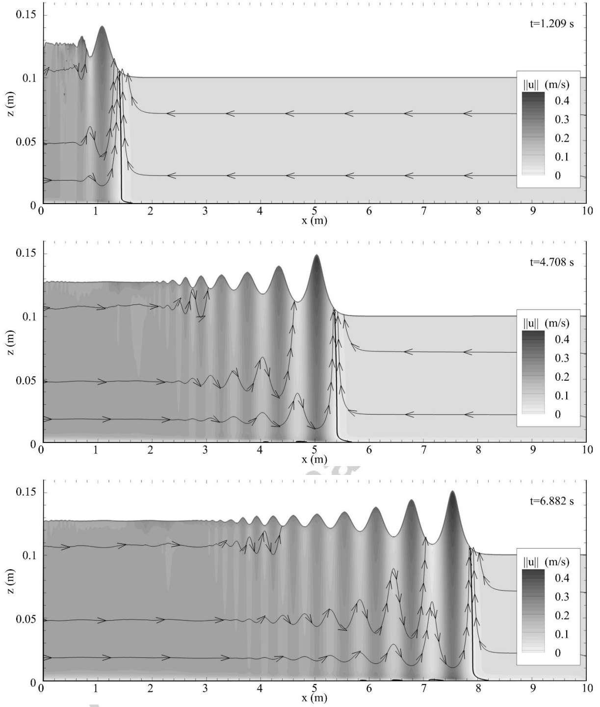
Fig. 8 Case D: dominated by bore flow, mapping of the velocity magnitude ||u|| in the water during bore propagation at 3 different times with velocity streamlines (lines with arrows) and the isoline of u_x = 0 (black lines). Axis scales are independent.
