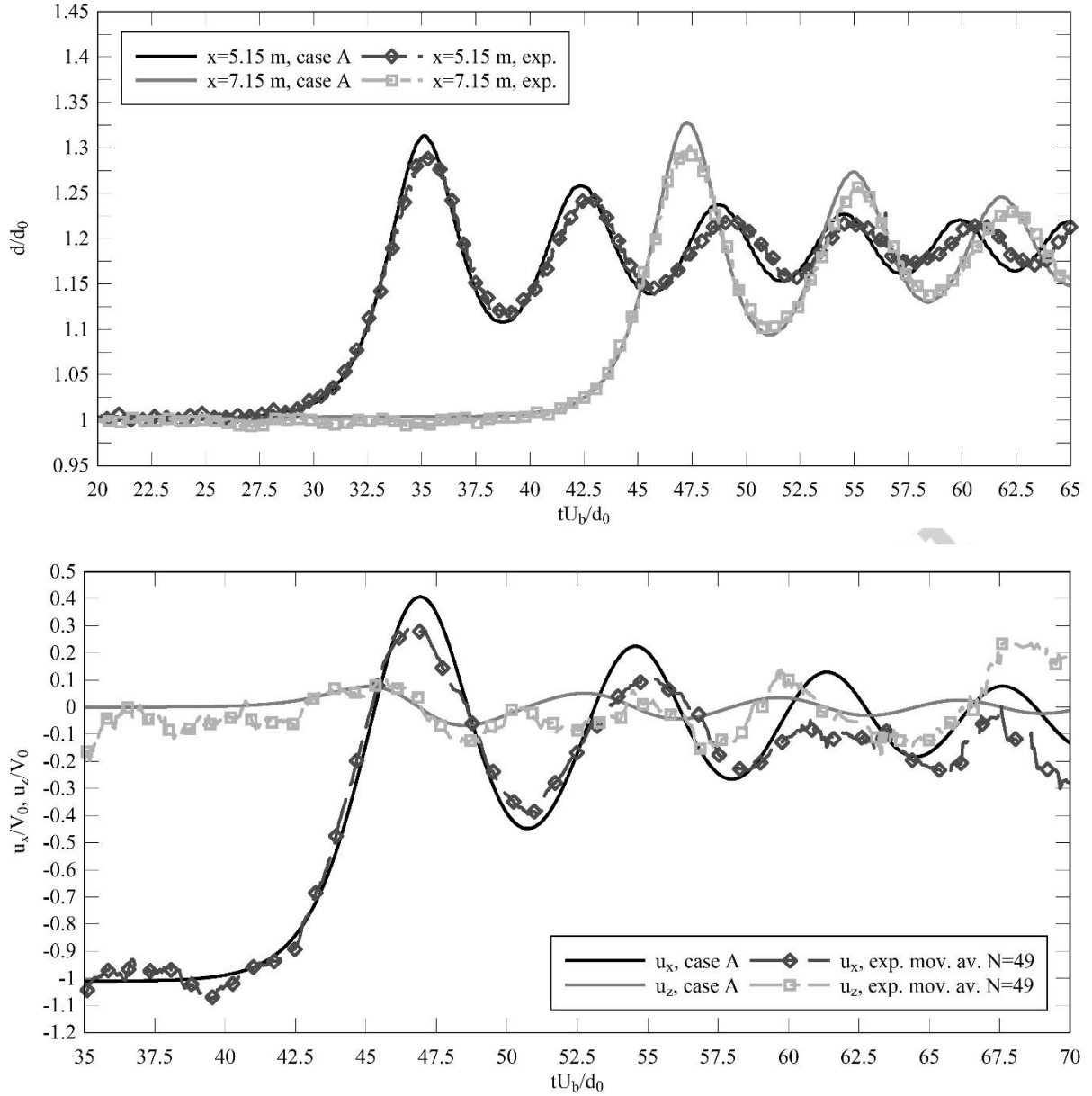
Fig. 3 Comparison between numerical simulations and experimental (exp) data. Top figure: time evolution of the free surface d/d_0 of undular bores where d_0 is the initial water depth. Bottom figure: time evolution of horizontal and vertical components of the flow velocity, u_x/V_0 and u_z/V_0 , at z/d_0 = 0.18 with V_0 the initial velocity (where mov. av. = moving average and N = number of measured data).
