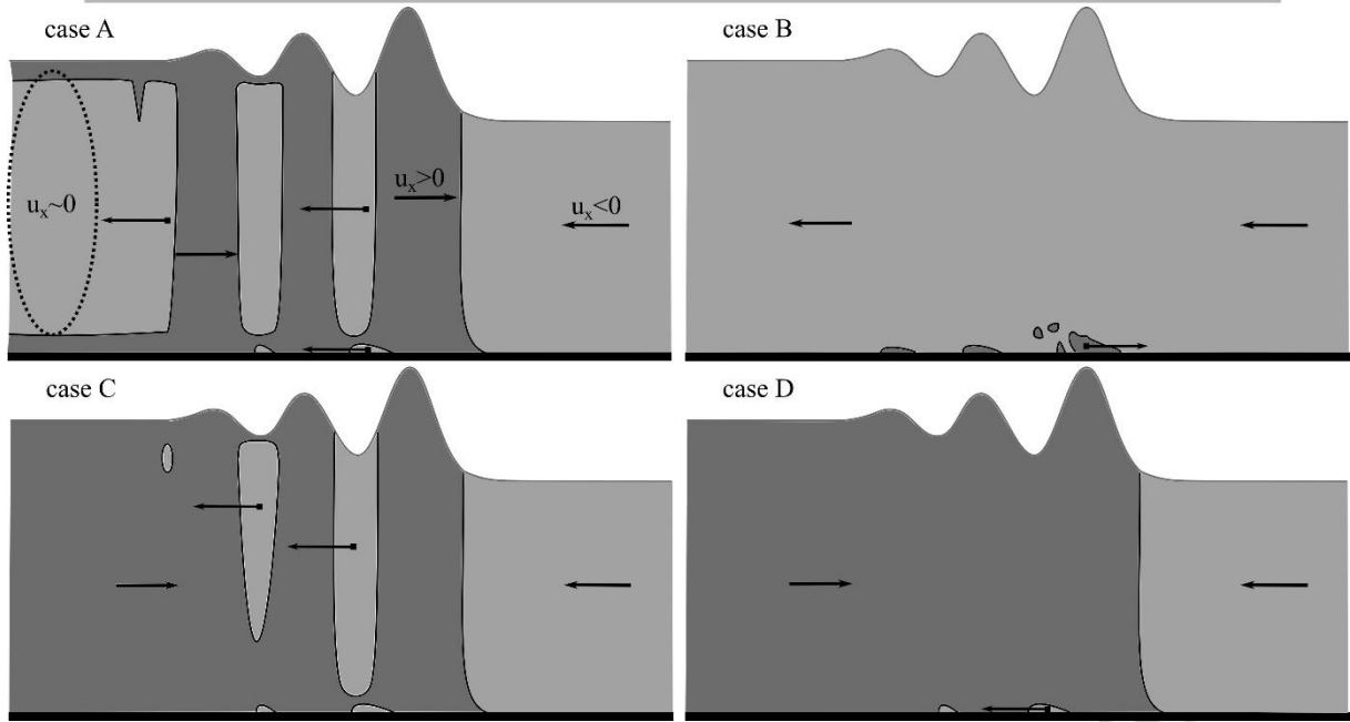
Fig. 9 Simplified schemes of the longitudinal component of the flow velocity when the bore is developed. Focus on the bore front and its first stubbles. The dark gray area represents a region with u_x > 0 and the light gray area represents u_x < 0 . The black lines are for u_x = 0 .
