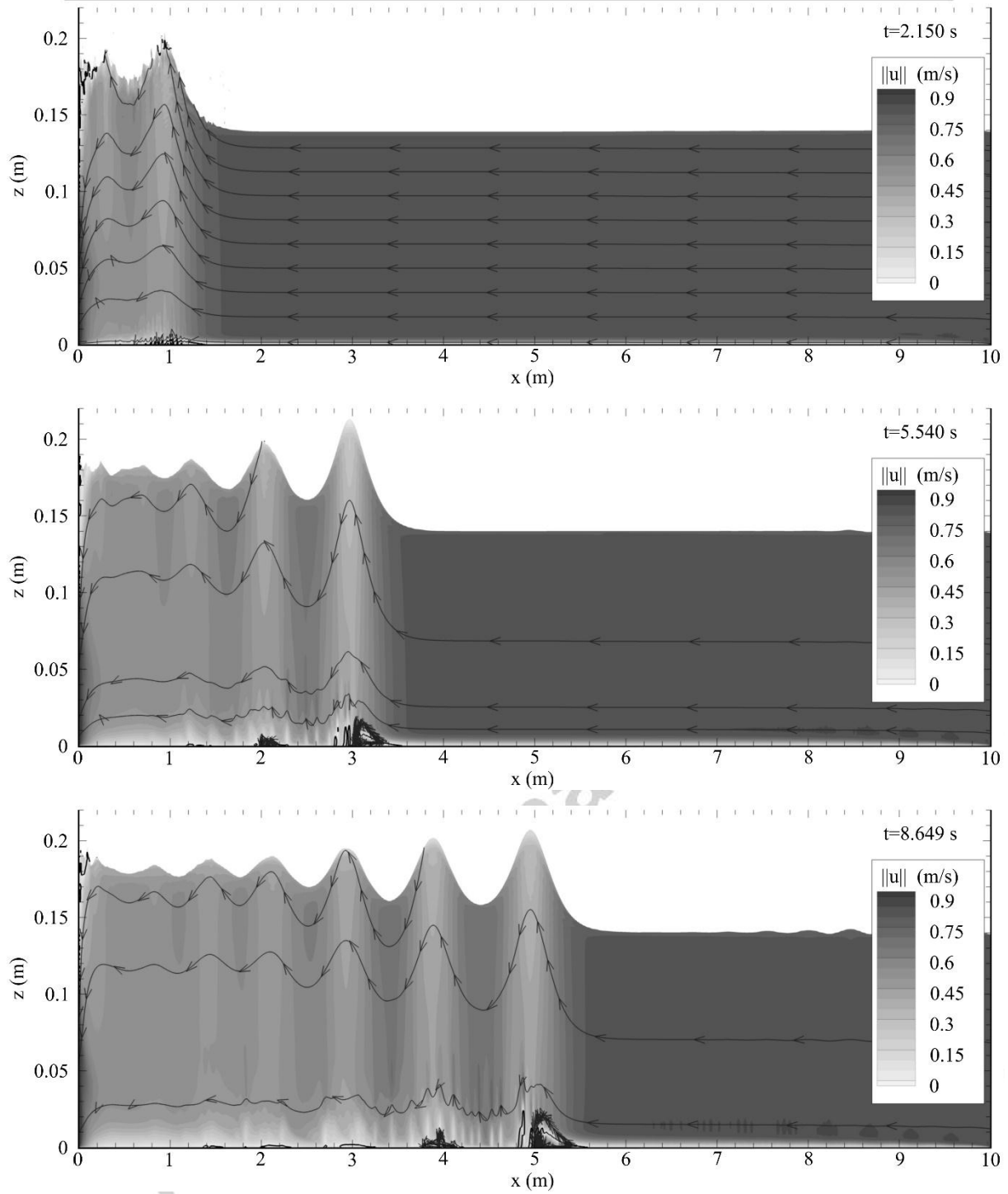
Fig. 5 Case B: dominated by the initial current, mapping of the velocity magnitude \|\mathbf{u}\| in the water during the bore propagation at 3 different times with velocity streamlines (lines with arrows) and the isoline u_x = 0 (black lines). Axis scales are independent.
