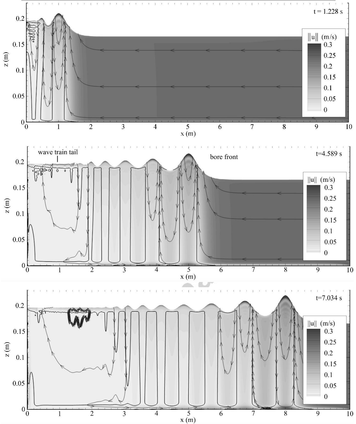
Fig. 4 Case A: dominated by undulations, mapping of the velocity magnitude \|\mathbf{u}\| in the water during the bore propagation at 3 different times with velocity streamlines (lines with arrows) and the isoline u_x = 0 (black lines). Axis scales are independent.
