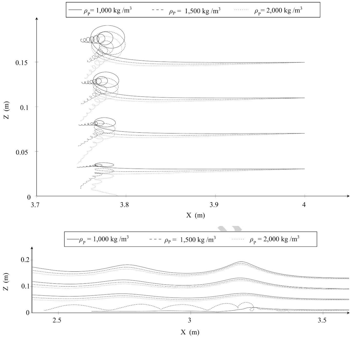
Fig. 10 Trajectories of suspended particles during the passage of the bore at different injection heights and different densities (Top: Case A and Bottom: Case B).
