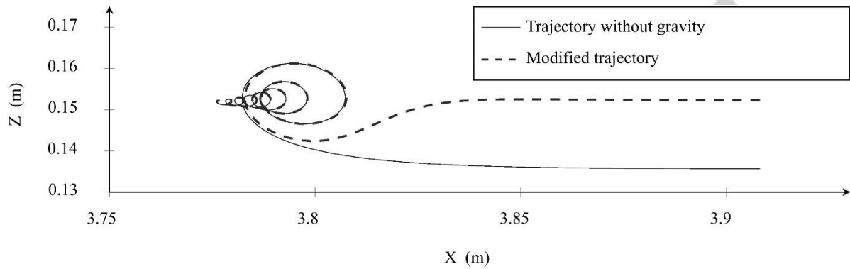
Fig. 15 Comparison of the full trajectory to the one whose contribution due to gravity was removed (Case A).
