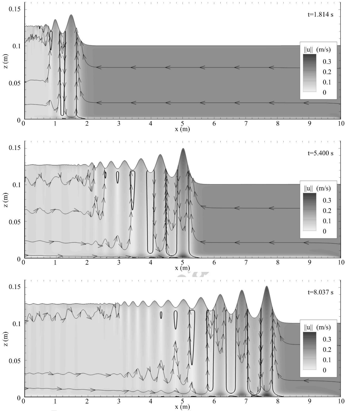
Fig. 7 Case C: partially dominated by undulations and then the bore flow, mapping of the velocity magnitude \|\mathbf{u}\| in the water during the bore propagation at 3 different times with velocity streamlines (lines with arrows) and the isoline of u_x = 0 (black lines). Axis scales are independent.
