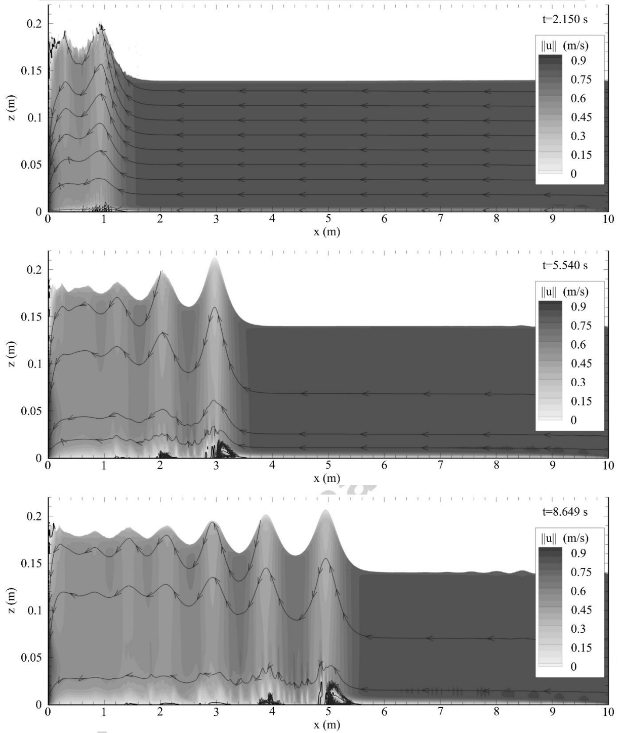
Fig. 5 Case B: dominated by the initial current, mapping of the velocity magnitude \|u\| in the water during the bore propagation at 3 different times with velocity streamlines (lines with arrows) and the isoline u_x = 0 (black lines). Axis scales are independent.
