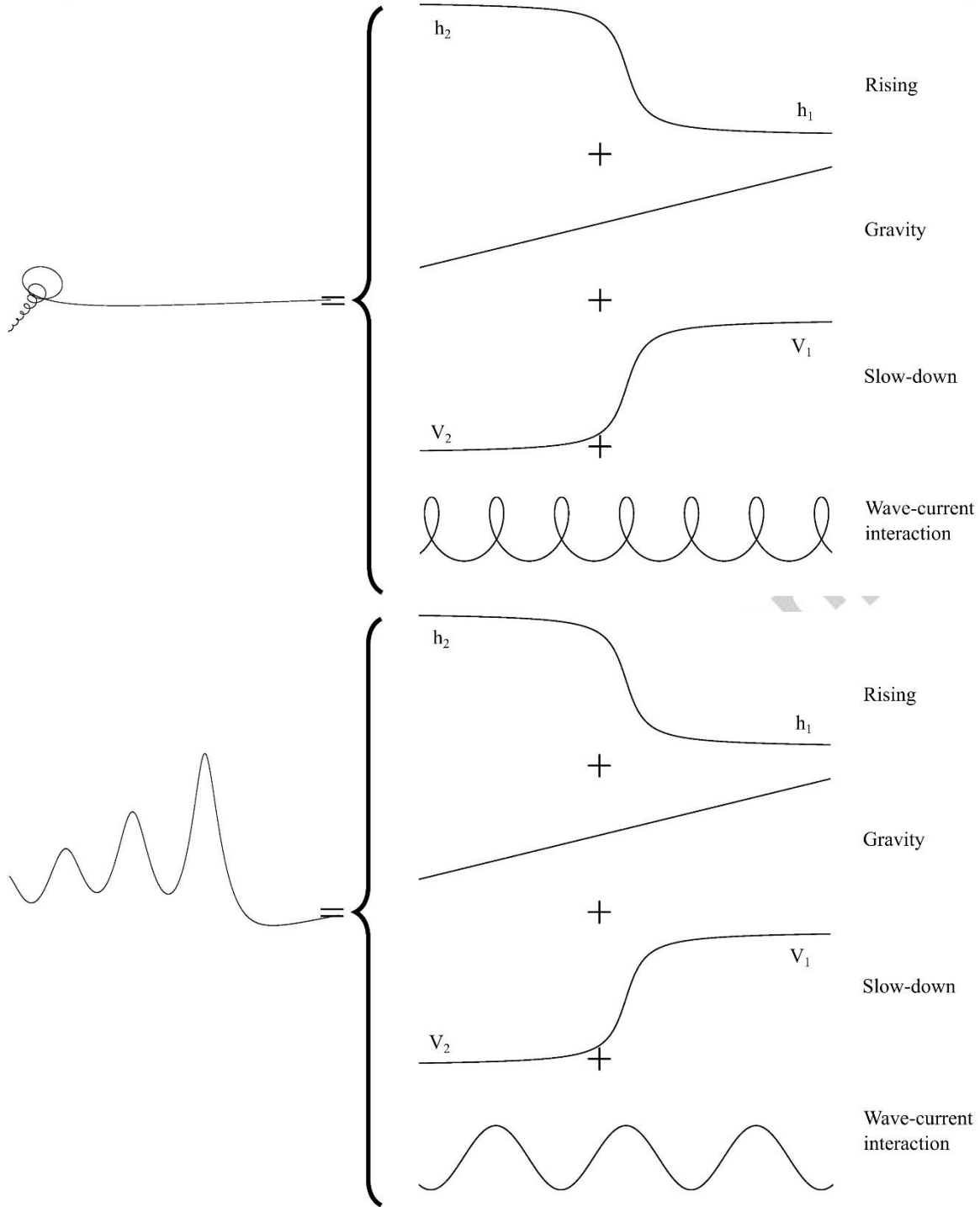
Fig. 14 The features of trajectories encountered in the two cases studied without reversal (Top: Case A and Bottom: Case B).
