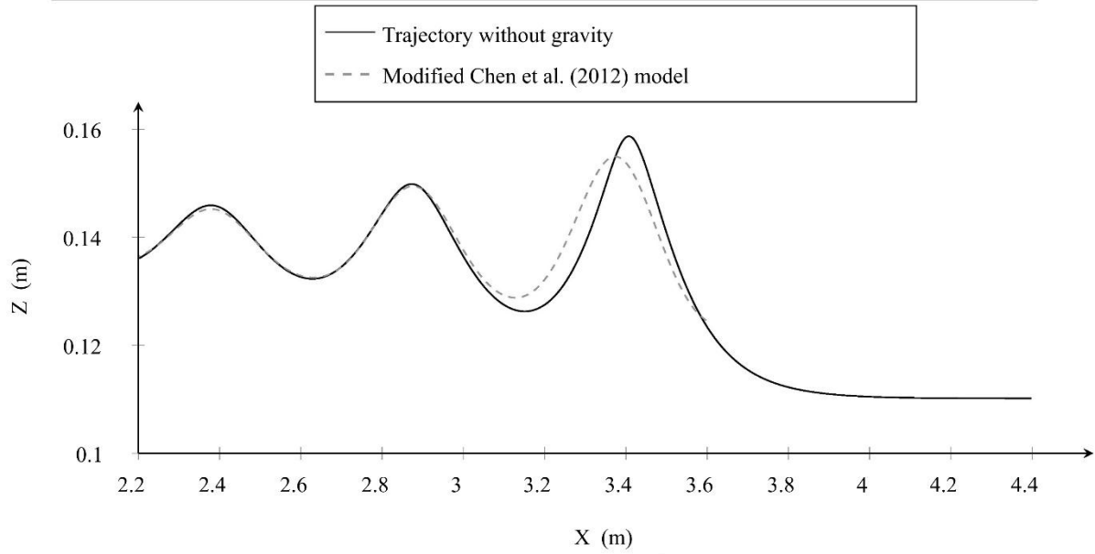
Fig. 20 Comparison of the trajectory without the contribution of gravity in the area following the passage of the bore front to the trajectory deduced from the wave-current interaction model including attenuation (Case B).
