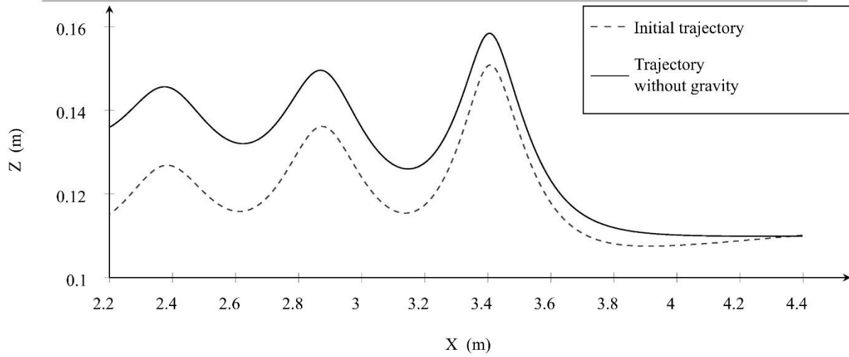
Fig. 18 Comparison of the full particle trajectory to the one with the contribution of gravity removed (Case B).
