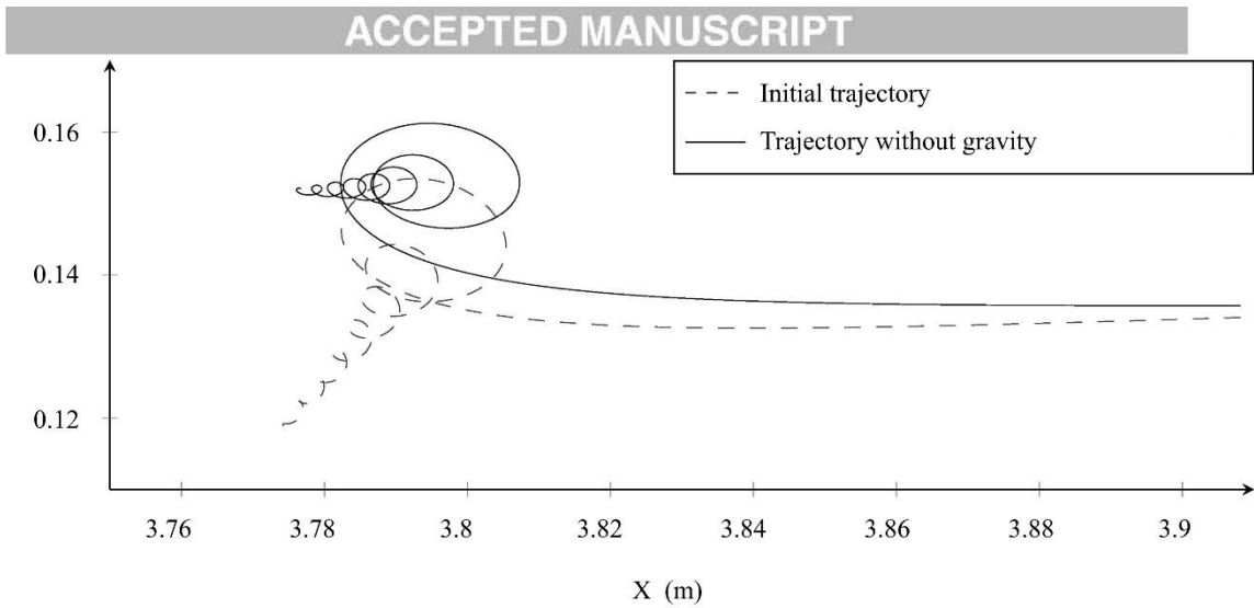
Fig. 15 Comparison of the full trajectory to the one whose contribution due to gravity was removed (Case A).
