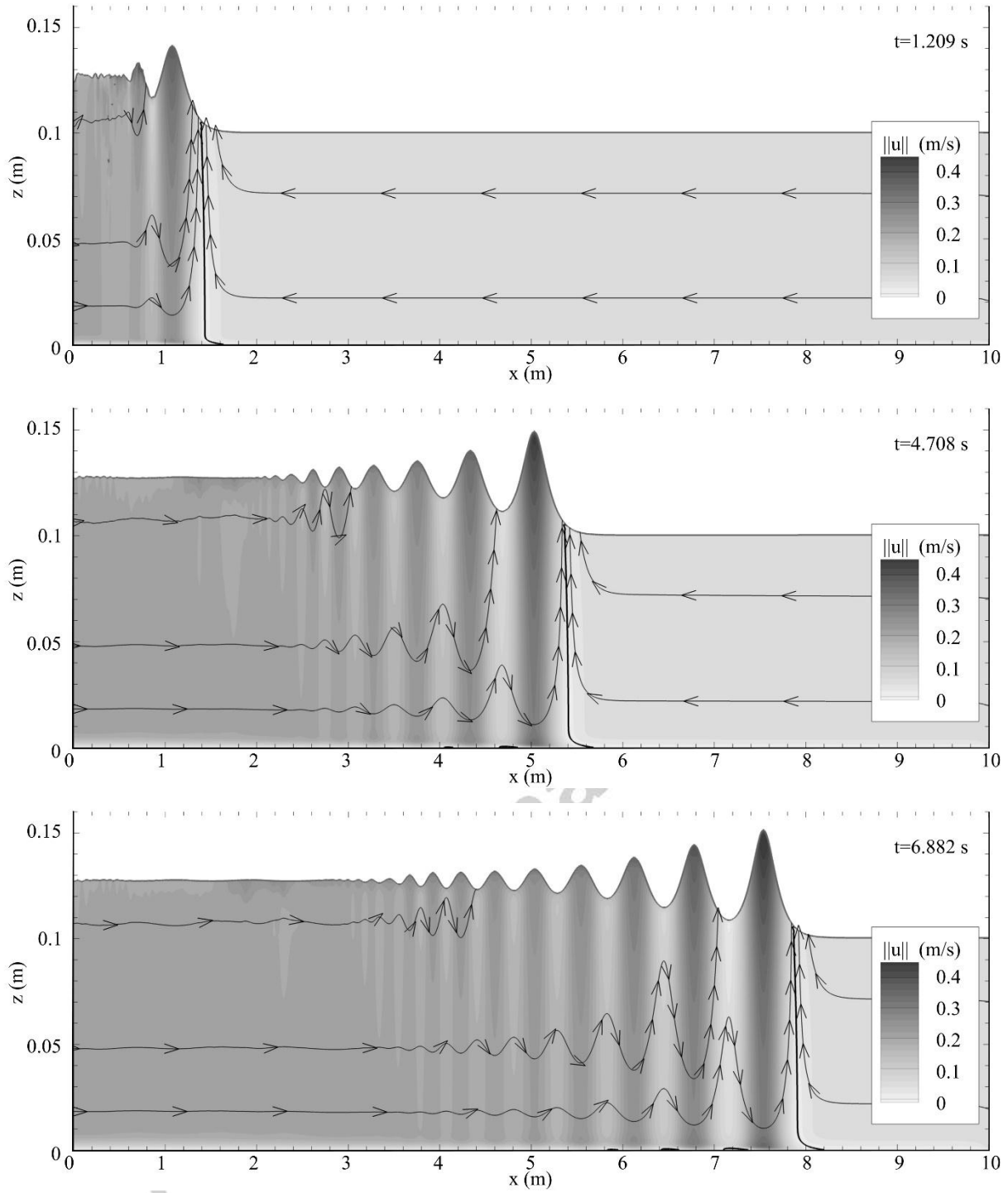
Fig. 8 Case D: dominated by bore flow, mapping of the velocity magnitude \|\mathbf{u}\| in the water during bore propagation at 3 different times with velocity streamlines (lines with arrows) and the isoline of u_x = 0 (black lines). Axis scales are independent.
