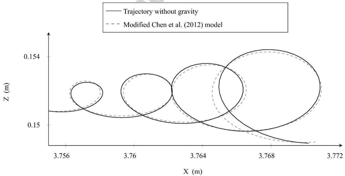
Fig. 16 Comparison of the trajectory without the contribution of gravity to the trajectory where the contributions of gravity, elevation, and the slowing down have been removed (Case A).
