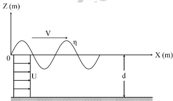
Fig. 21 Diagram showing a continuous wave train propagating on a uniform current.
